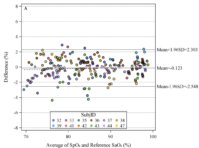
P-SP01 sensor accuracy, non-motion
