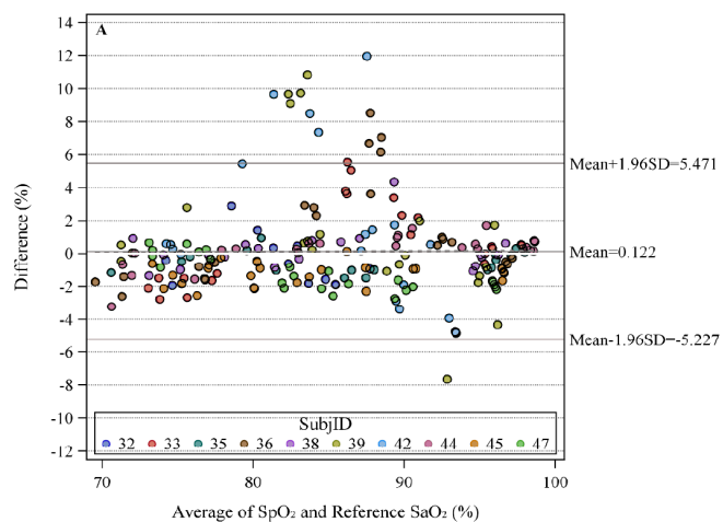
P-SP01 sensor accuracy, motion
