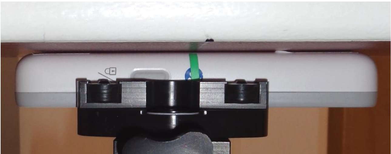
Back side of the HUB against the phantom, 0mm separation distance
