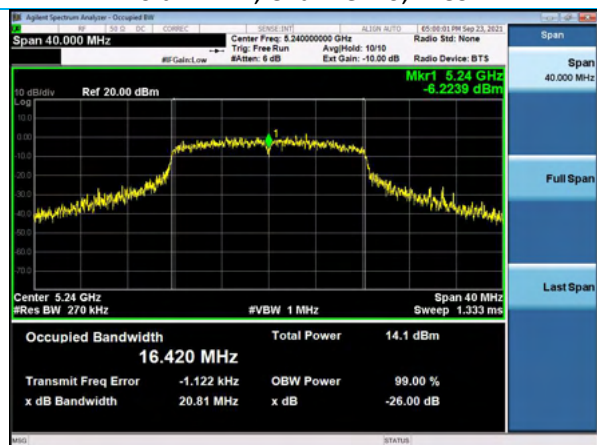
26 dB EBW, Channel 48, 54Mbps
