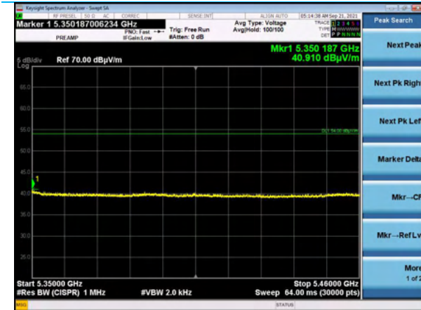
5350-5460 MHz, Channel 48, MCS0, Average Vertical Antenna
