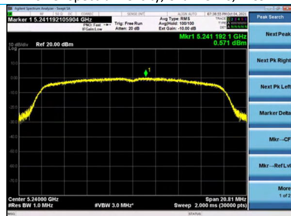
Power Spectral Density, Channel 48, 54Mbps
