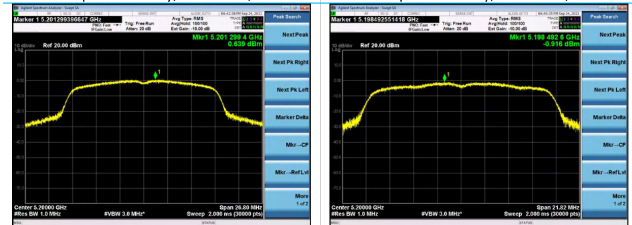
Power Spectral Density, Channel 40, 6Mbps
