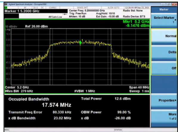
26 dB EBW, Channel 40, MCS7
