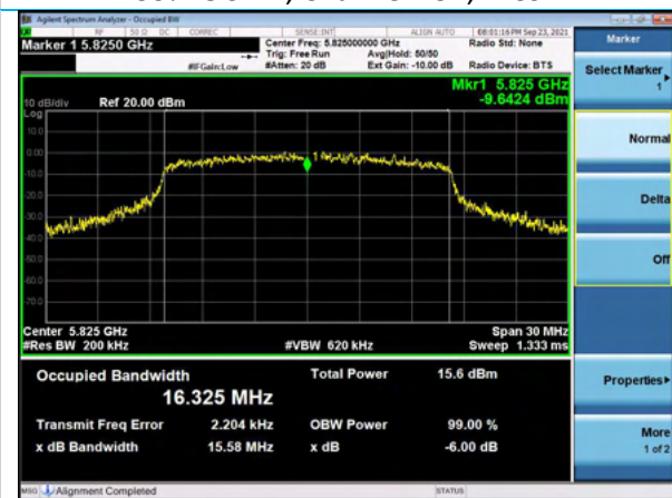
99% OCBW, Channel 165, 54Mbps
