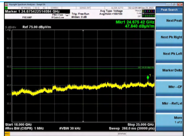
18-25 GHz, Channel 149, MCS0, Peak Vertical Antenna
