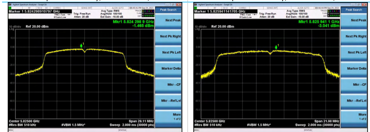
Power Spectral Density, Channel 165, 6Mbps
