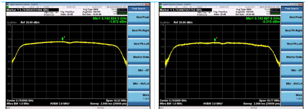
Power Spectral Density, Channel 149, 6Mbps
