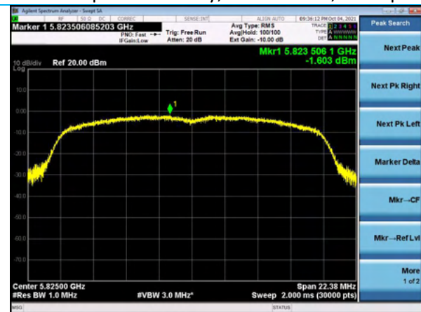
Power Spectral Density, Channel 165, MCS7
