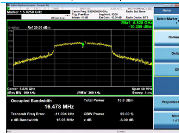
DTS BW, Channel 165, 6Mbps
