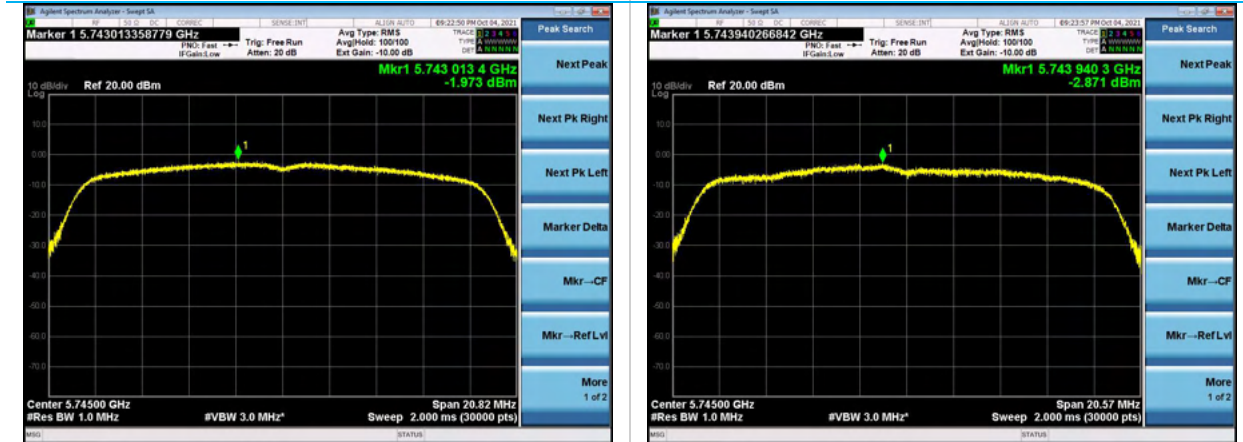
Power Spectral Density, Channel 149, MCS0
