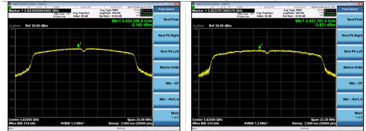
Power Spectral Density, Channel 165, MCS0
