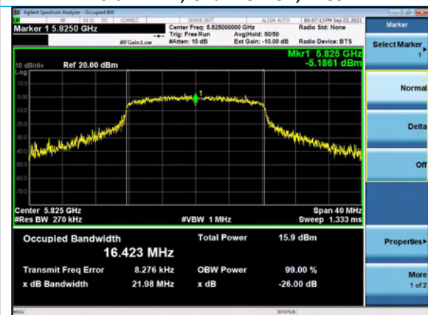
26 dB EBW, Channel 165, 54Mbps
