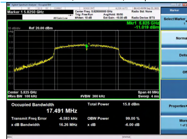
DTS BW, Channel 165, MCS0
