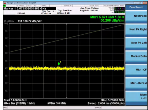
5650-5700 MHz, Channel 165, MCS0, Peak Vertical Antenna
