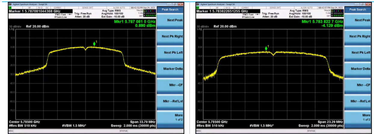
Power Spectral Density, Channel 157, MCS0
