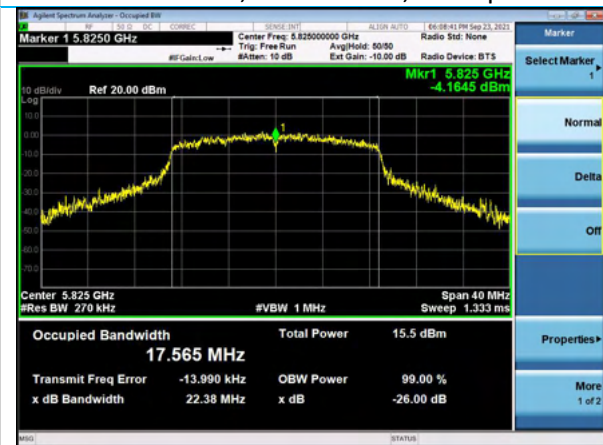
26 dB EBW, Channel 165, MCS7
