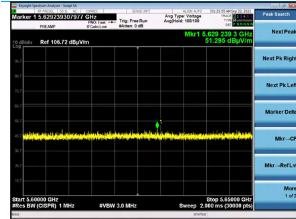
5600-5650 MHz, Channel 157, MCS0, Peak Vertical Antenna
