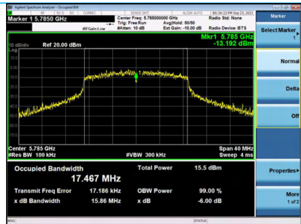
DTS BW, Channel 157, MCS7
