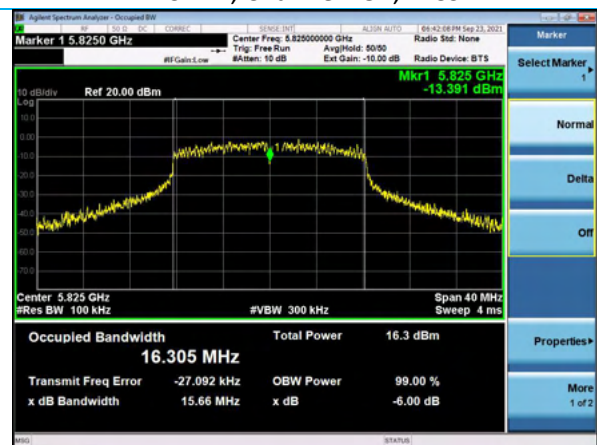
DTS BW, Channel 165, 54Mbps
