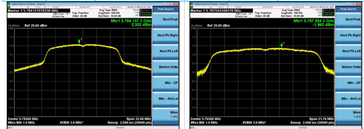
Power Spectral Density, Channel 157, 6Mbps
