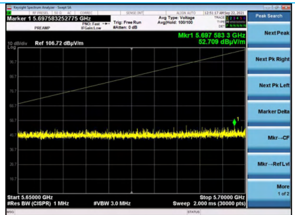
5650-5700 MHz, Channel 149, MCS0, Peak Vertical Antenna
