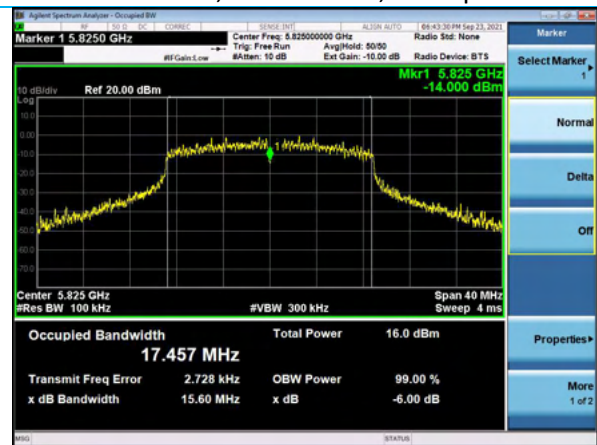
DTS BW, Channel 165, MCS7
