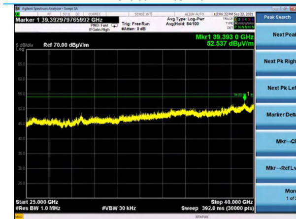
25-40 GHz, Channel 149, MCS0, Peak Vertical Antenna
