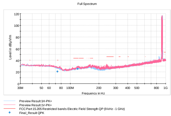
Figure 11: Result 30 – 1000 MHz
