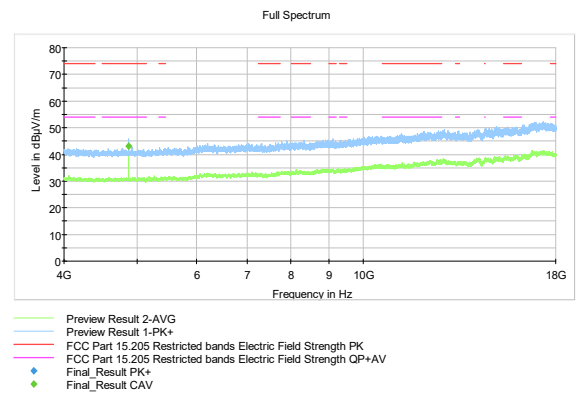
Figure 8: MID channel b mode (4 GHz – 18 GHz)
