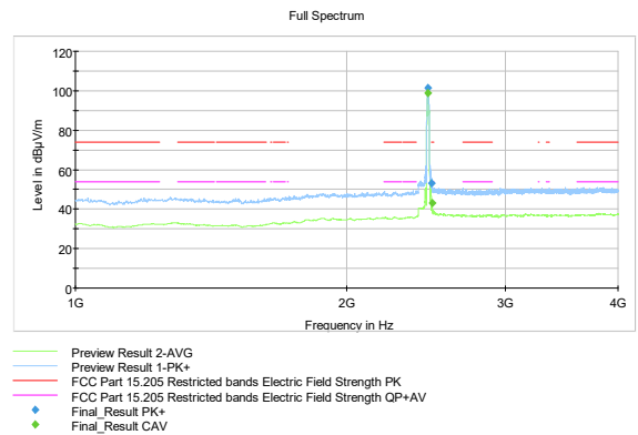
Figure 11: HIGH channel b mode (1 GHz – 4 GHz)
