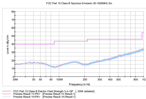
Figure 10: HIGH channel b mode (30 MHz – 1000 MHz)
