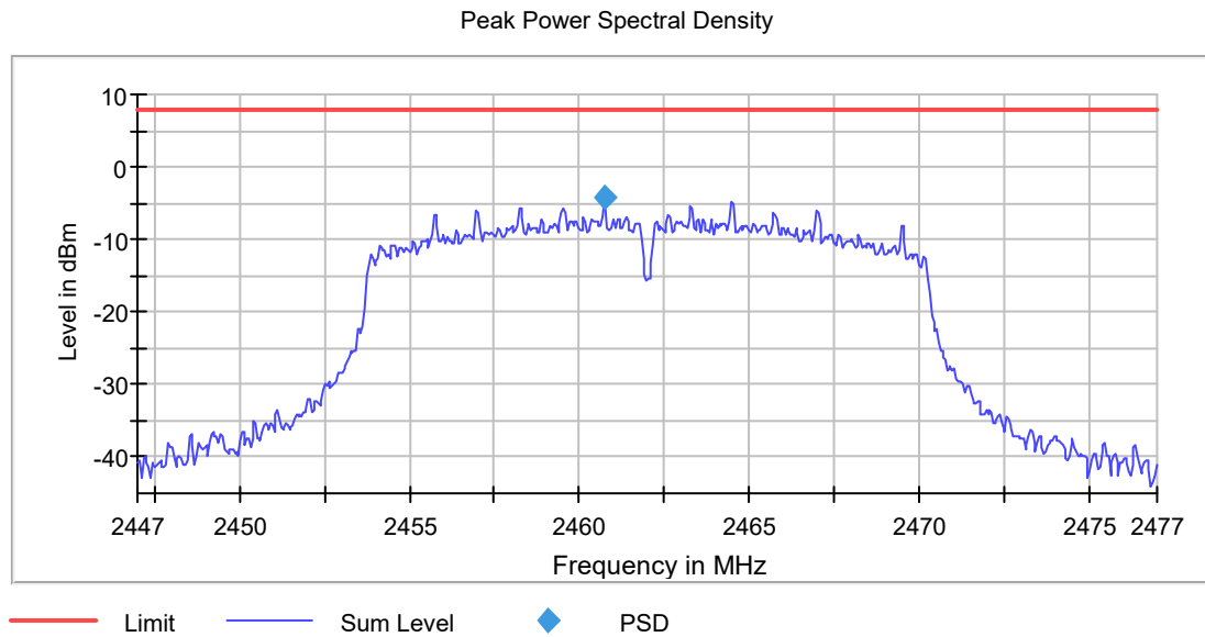
Figure 20: Power spectral density, channel HIGH, g mode
