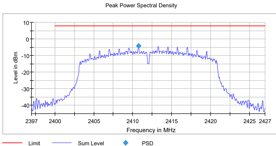
Figure 21: Power spectral density, channel LOW, n mode
