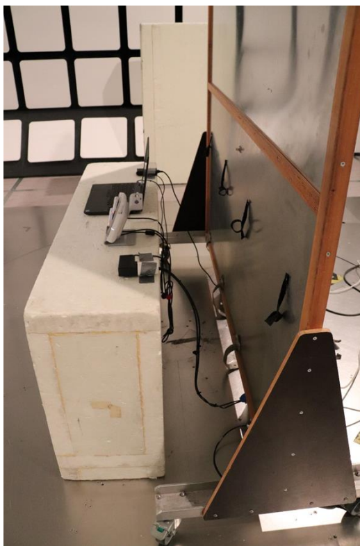
Photograph 6. Test Setup for Conducted Emissions 150 kHz – 30 MHz
