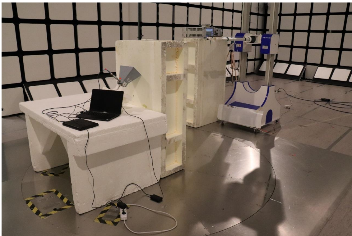
Photograph 5. Test Setup for Radiated Emissions 26.5 – 40 GHz
