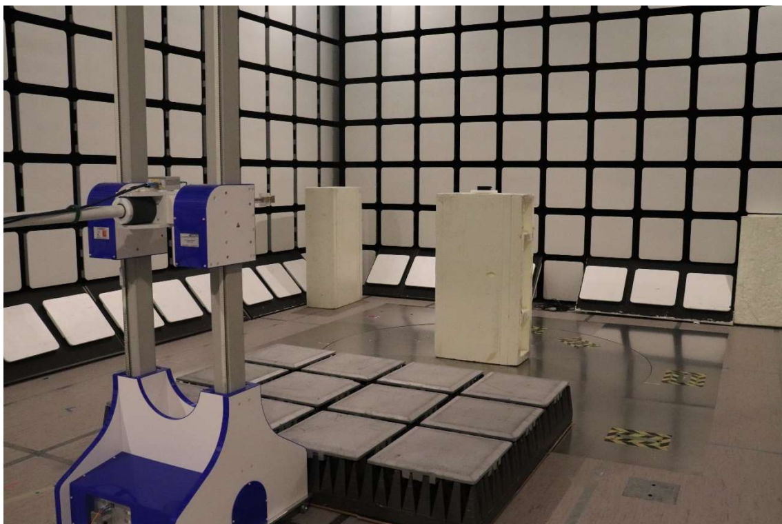
Photograph 4. Radiated emission 18 – 26.5 GHz
