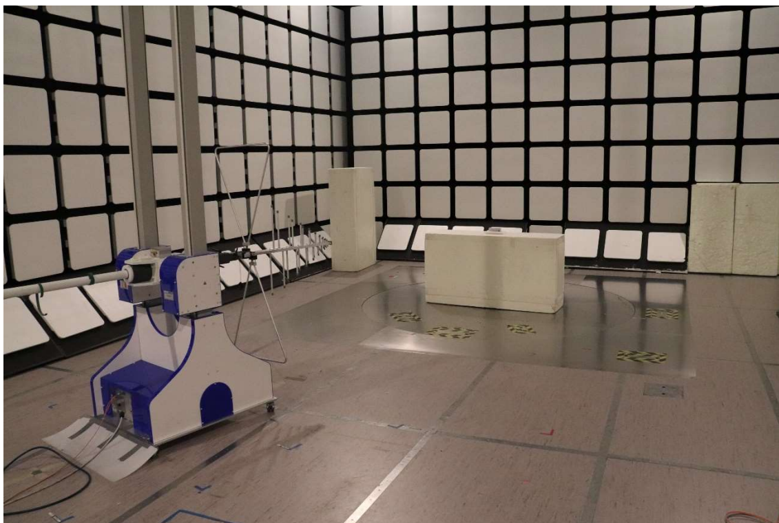
Photograph 2. Radiated emission 30 - 1000 MHz
