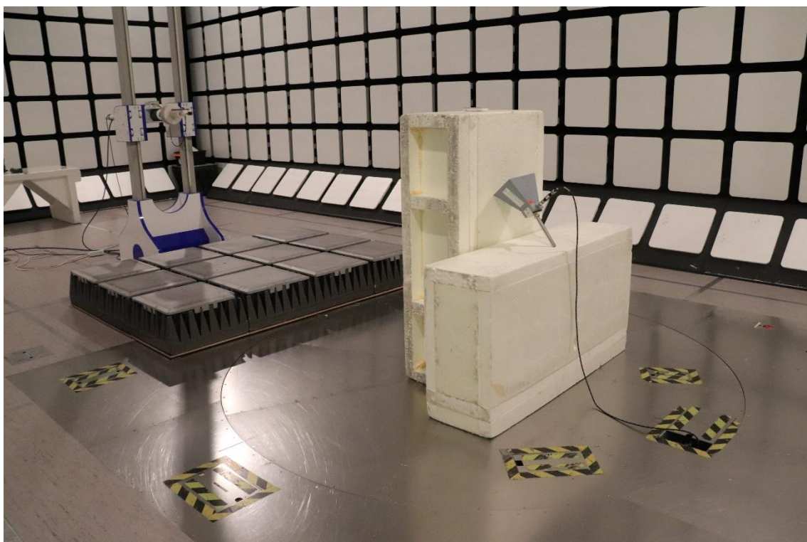
Photograph 4. Radiated emissions 18 – 26.5 GHz
