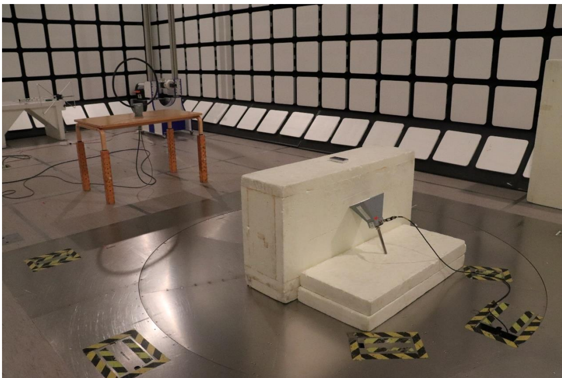
Photograph 1. Radiated emissions 9 kHz – 30 MHz
