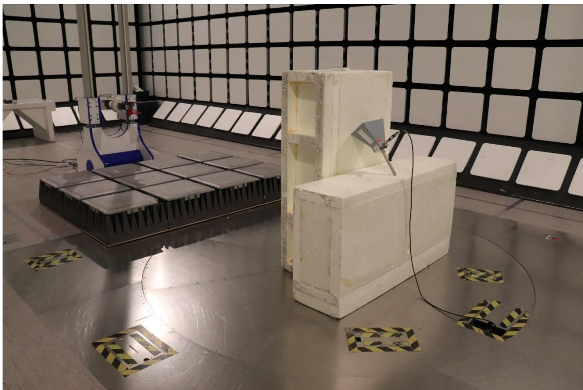
Photograph 3. Radiated emissions 1 – 18 GHz
