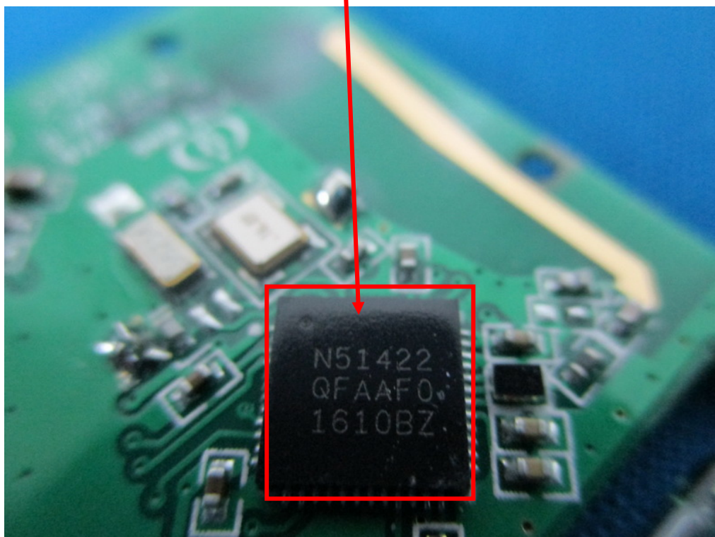
Bluetooth LE & ANT+ RF Chip IC – Top View
