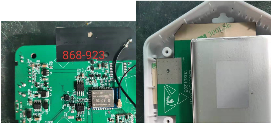
Antenna placement diagram
