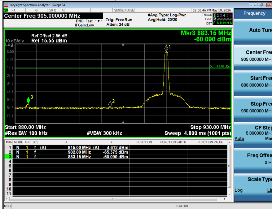
2 Bandedge_NVNT_ANT1_User_915
