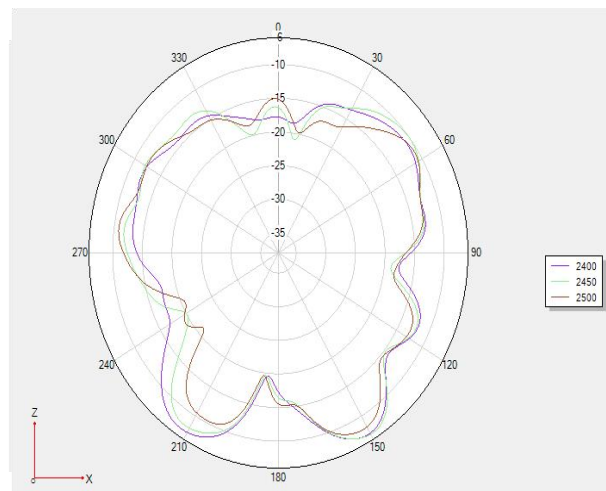
Phi 0 2D
