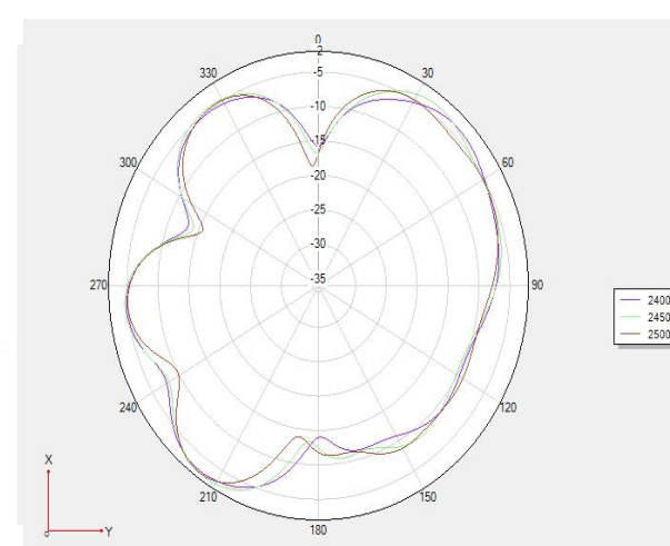
Theta 90 2D
