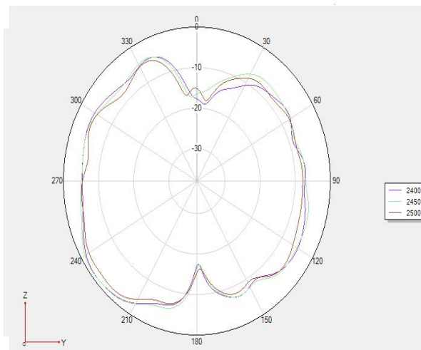
Phi 90 2D
