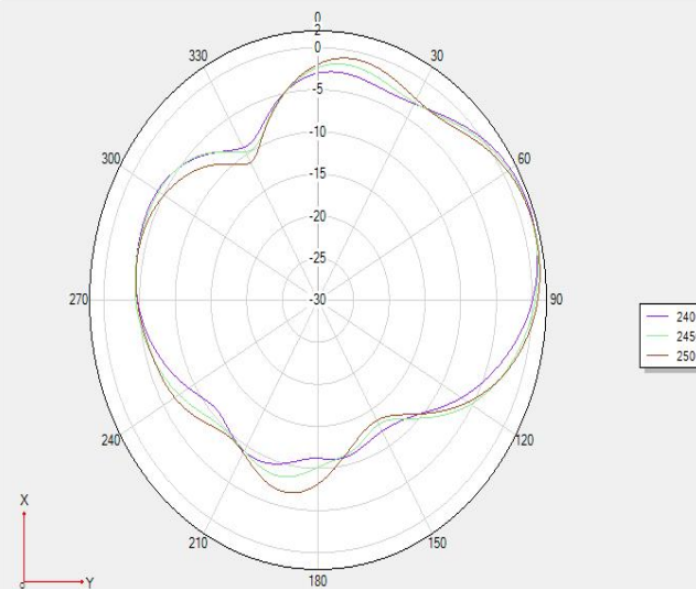
Theta 90 2D
