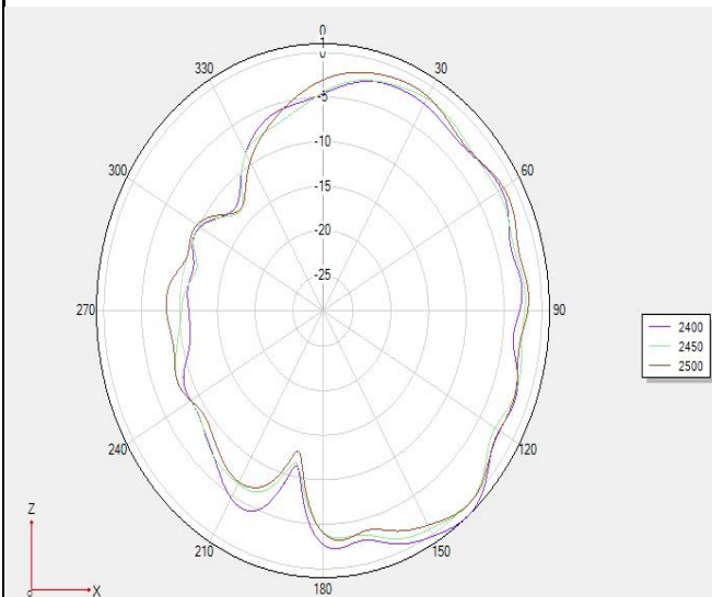
Phi 0 2D
