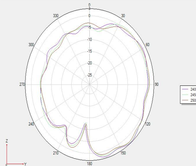
Phi 90 2D
