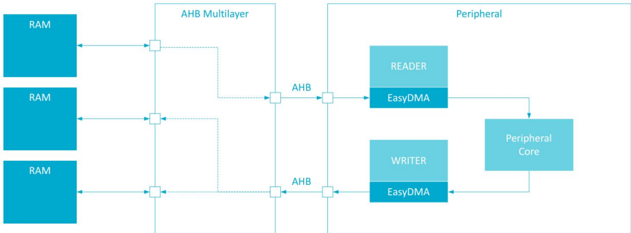
Figure 17: EasyDMA example
