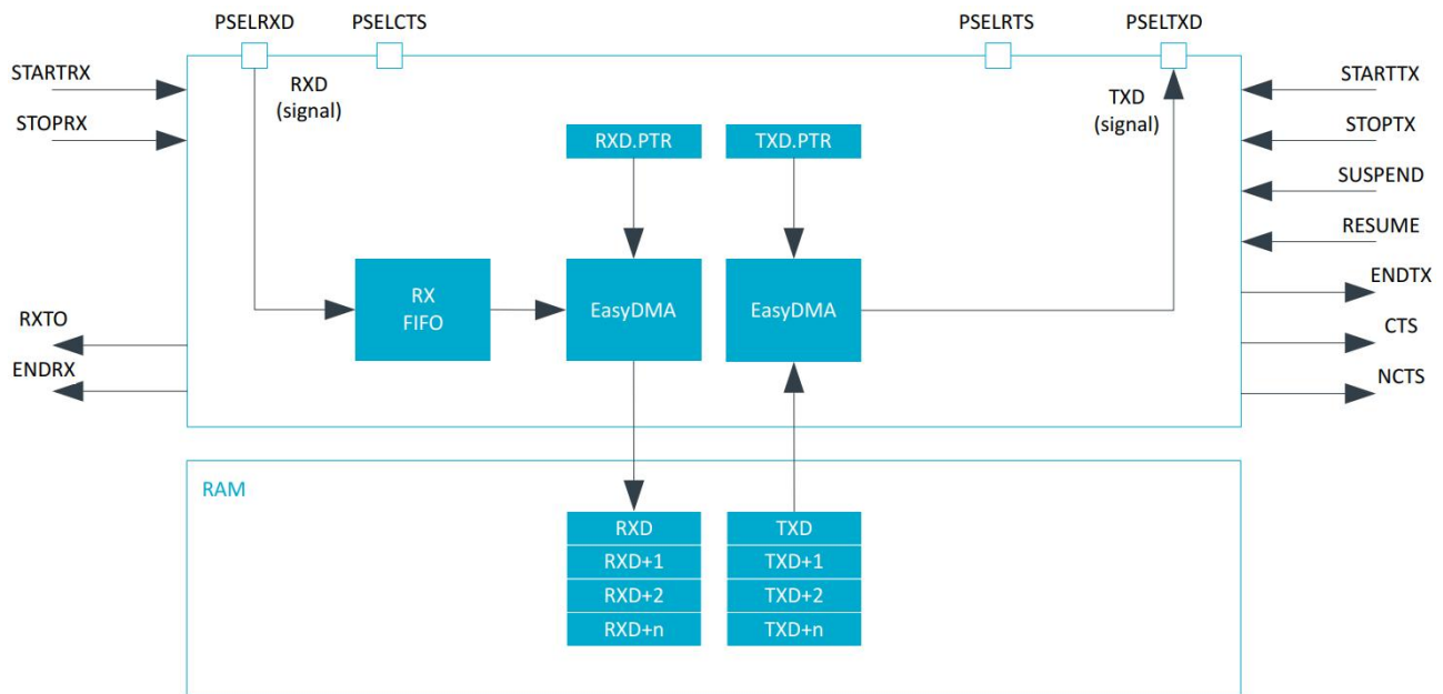
Figure 14: UART configuration
