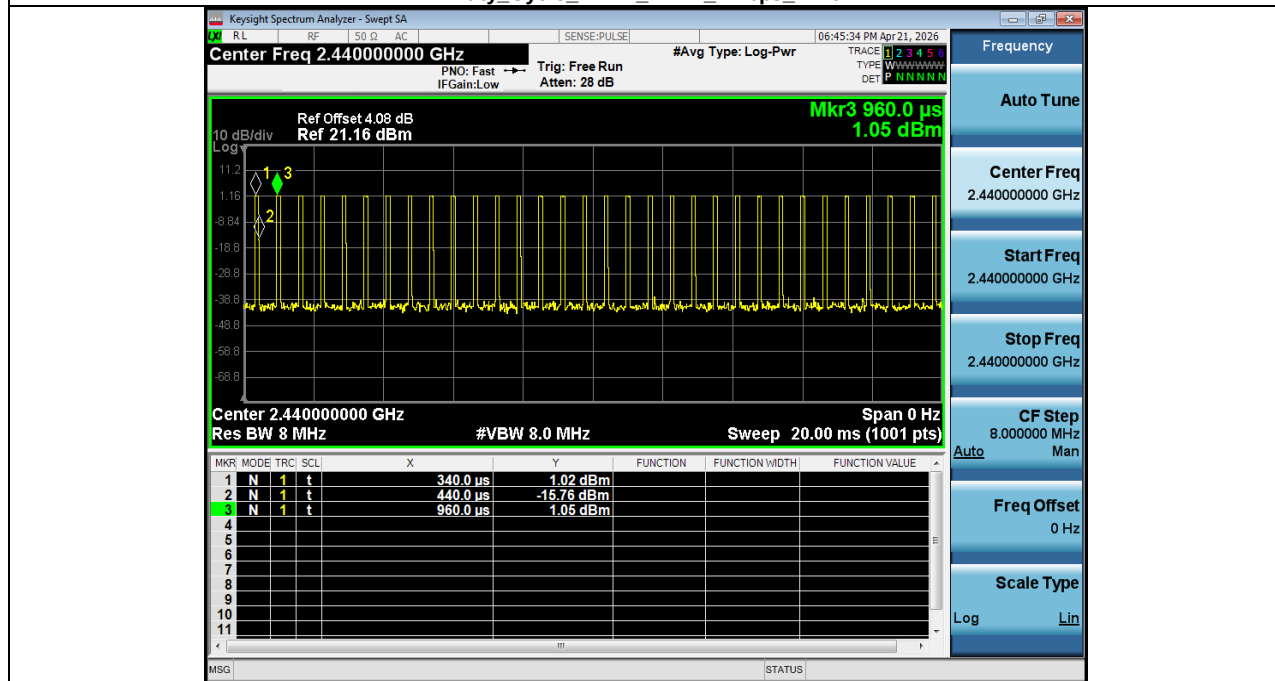
Duty Cycle_NVNT_ANT1_1Mbps_2440
