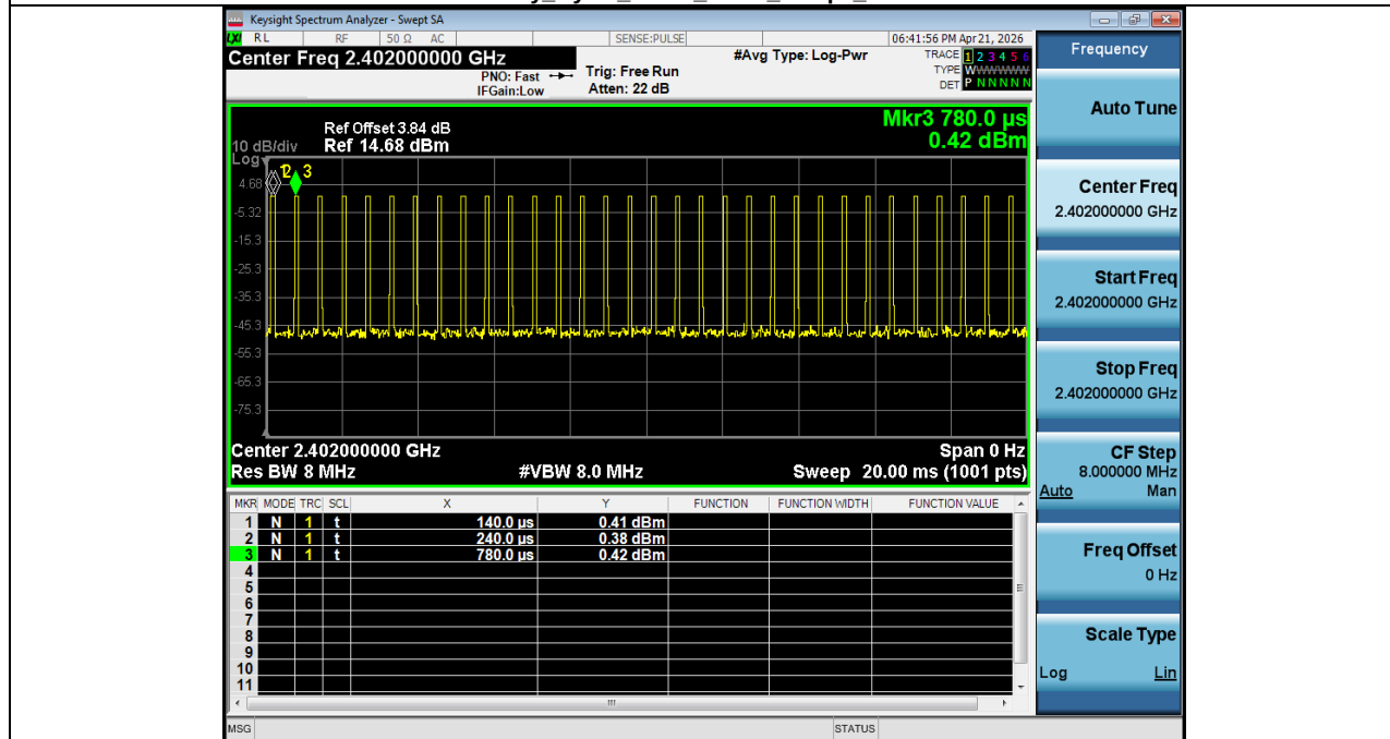
Duty Cycle_NVNT_ANT1_1Mbps_2402
