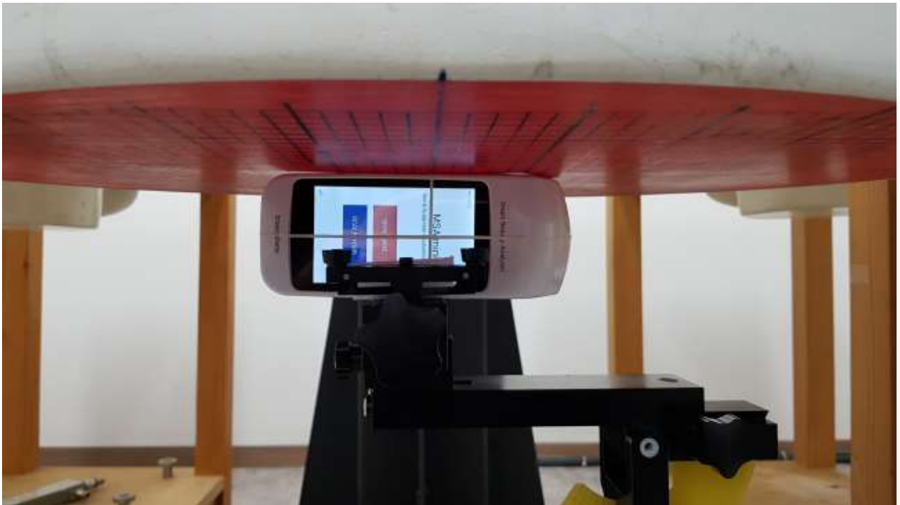
Front view (Left of DUT)
