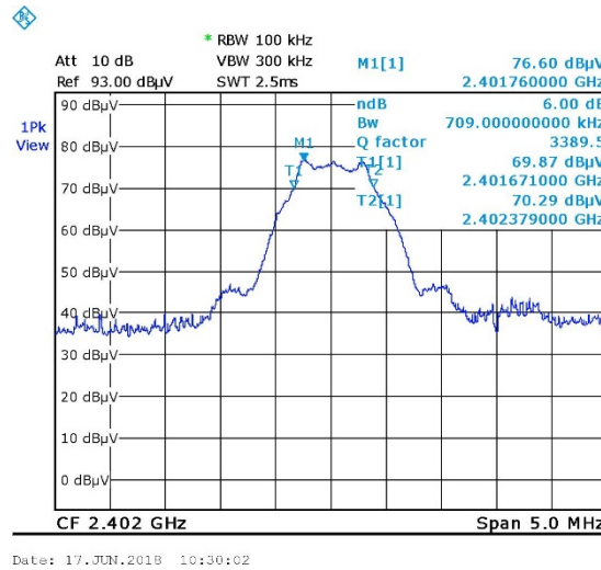
Figure 15. 2402.0 MHz
