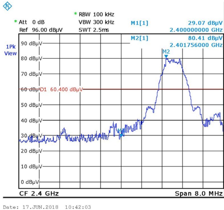
Figure 28 —Lower Band Edge
