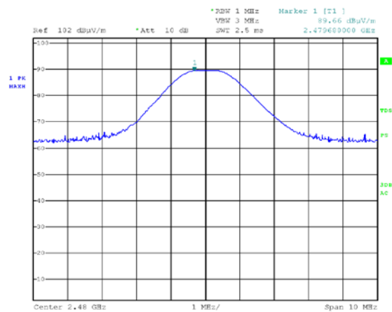
Figure 24 2480.0 MHz – Vertical
