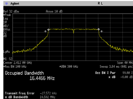
802.11g, 2412 MHz
