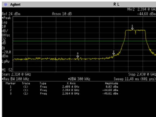
802.11g
