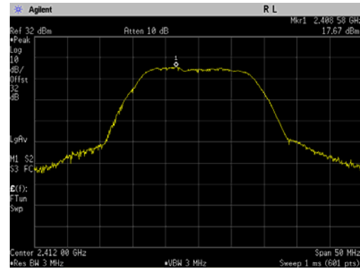
802.11g, 2412 MHz
