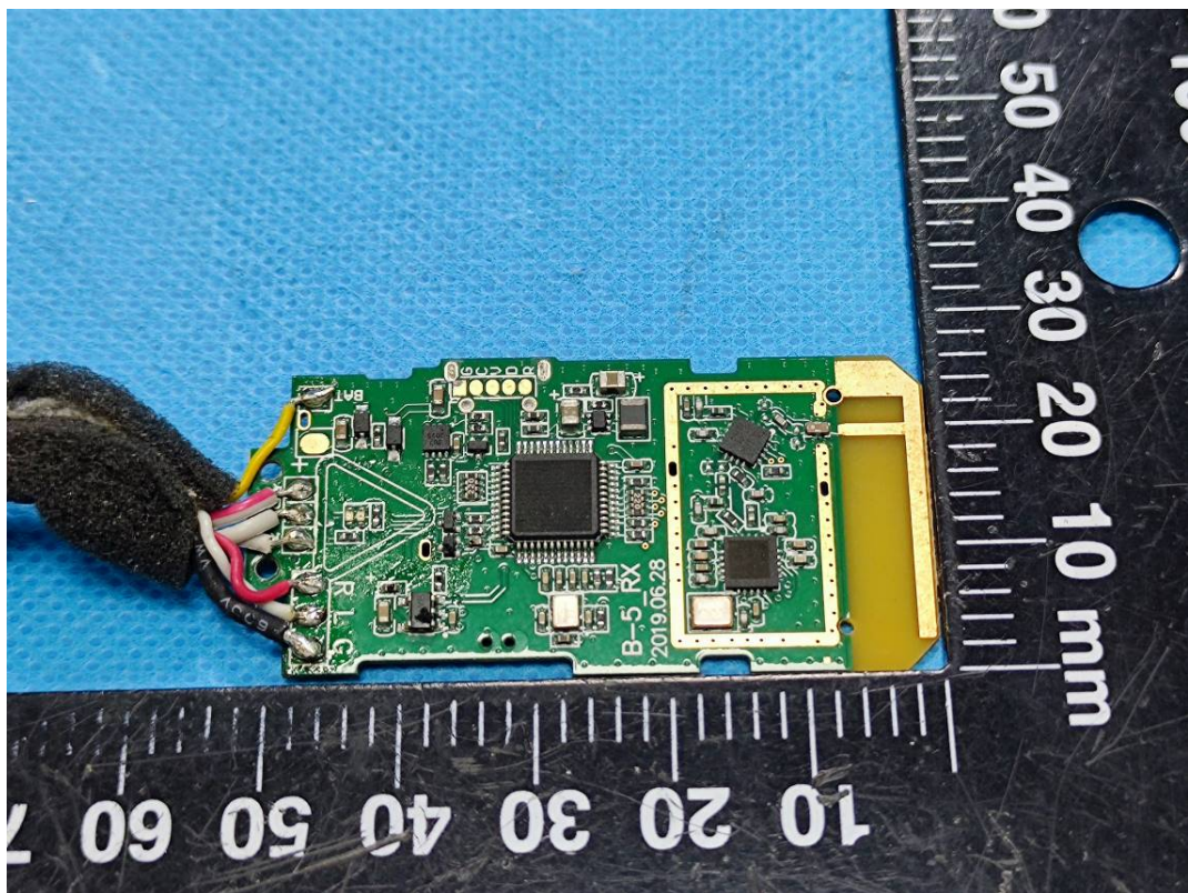
2.4G wireless RX module
