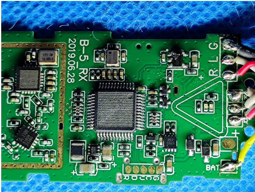
2.4G wireless RX module Antenna
