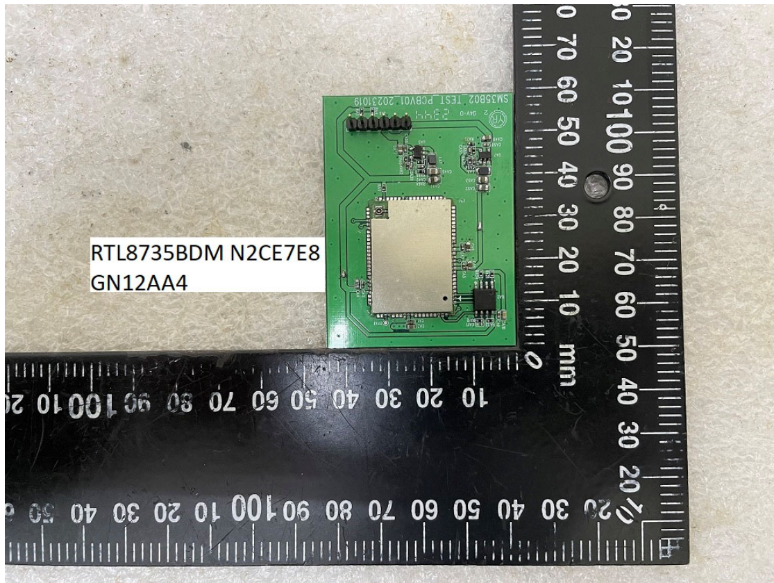
EUT-7. RTL8735BDM N2CE7E8 GN12AA4
