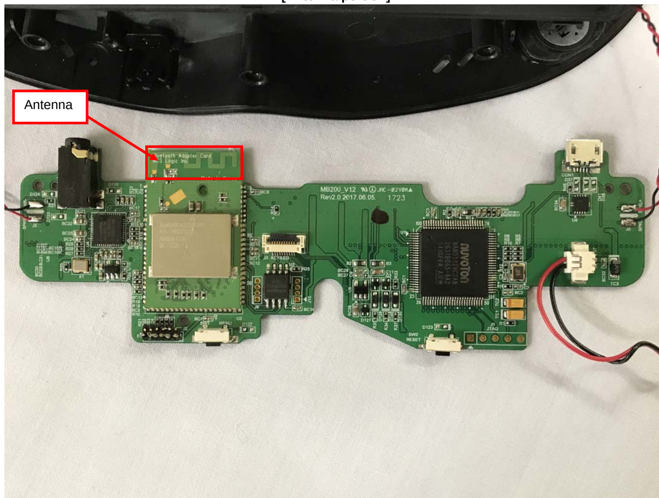
[Antenna portion]
