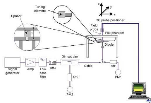
Fig 8.2 System Setup for System Evaluation
