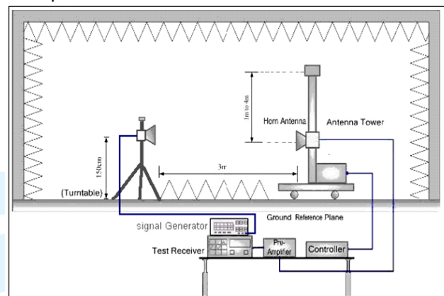
ERP Test Setup
