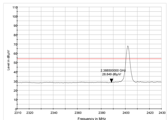
EDR -Channel 0: Average
