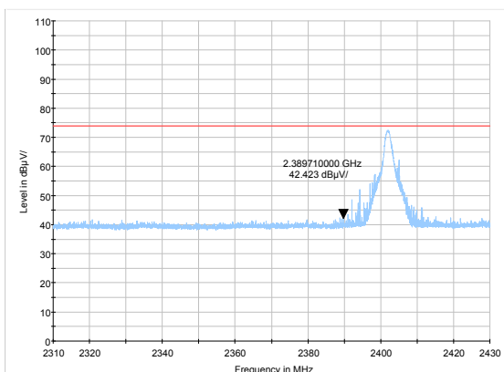
EDR -Channel 0: Peak
