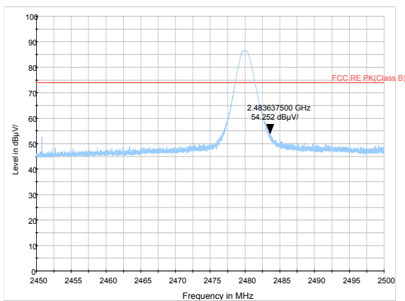
DH5-Channel 78: Peak
