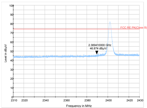
DH5-Channel 0: Peak
