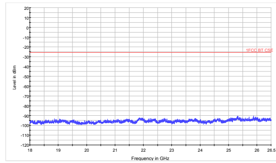
EDR-CH39 18GHz to 26.5GHz
