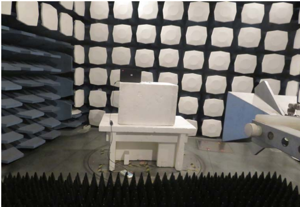
Above 1GHz
