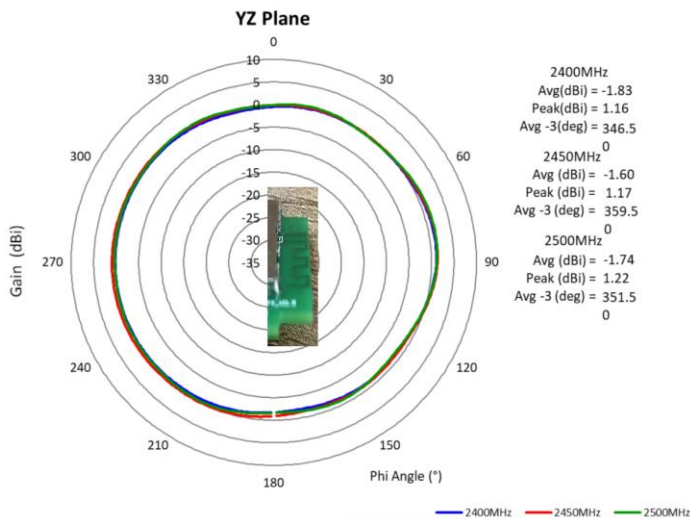
Radiation pattern Y-Z plane
