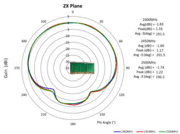
Radiation pattern Z-X plane
