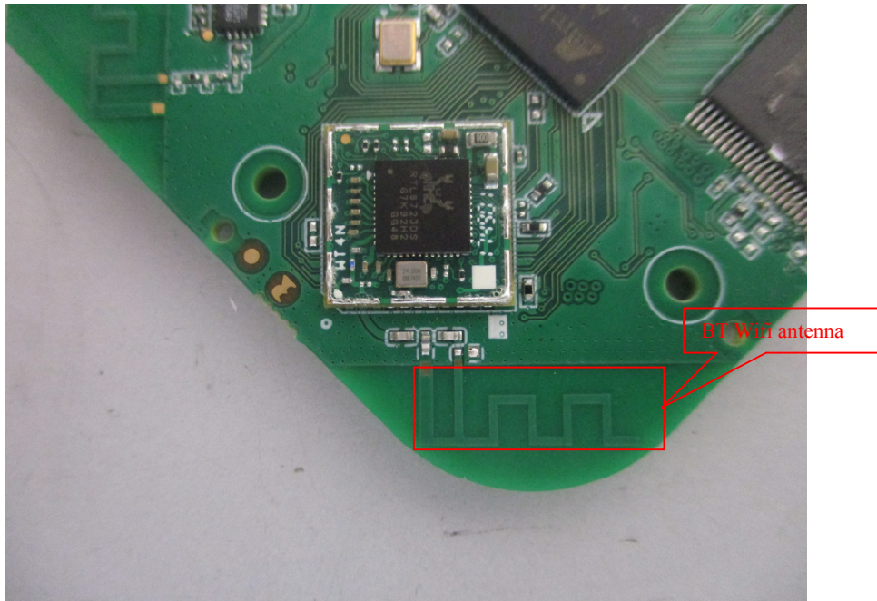
EUT – Antenna View-2
