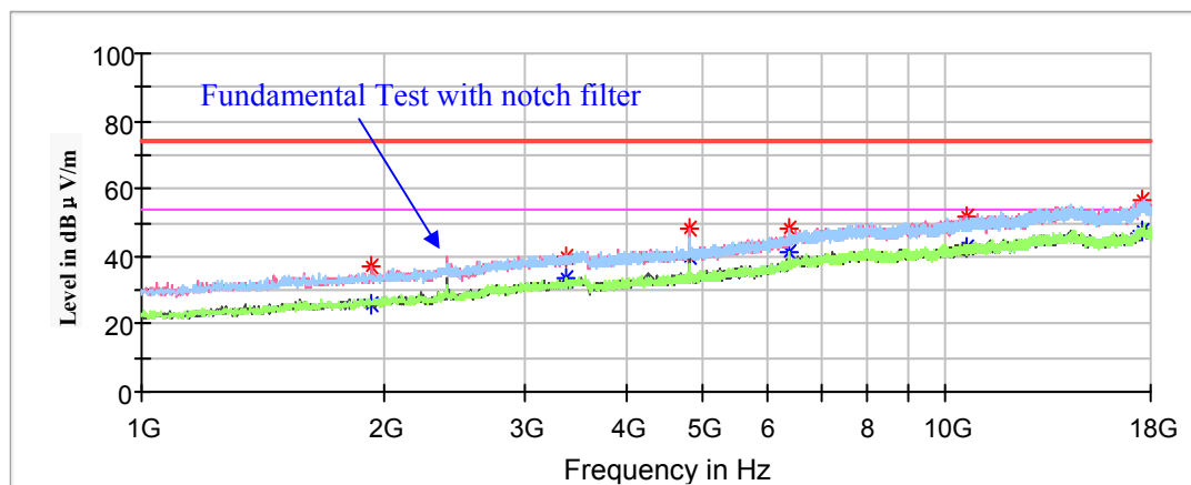
Full Spectrum
