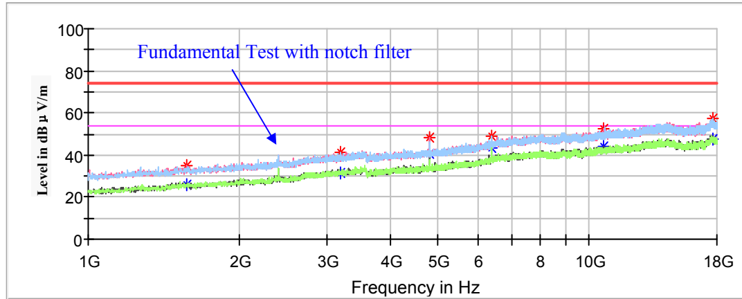
Full Spectrum
