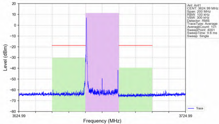
n48_30kHz_MIMO_NTNV_40MHz_CP-OFDM 16 QAM 3624.99MHz_Edge_1RB_Left_Ant1
