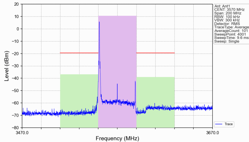
n48_30kHz_SISO_NTNV_40MHz_CP-OFDM 256 QAM 3570MHz_Edge_1RB_Left_Ant1
