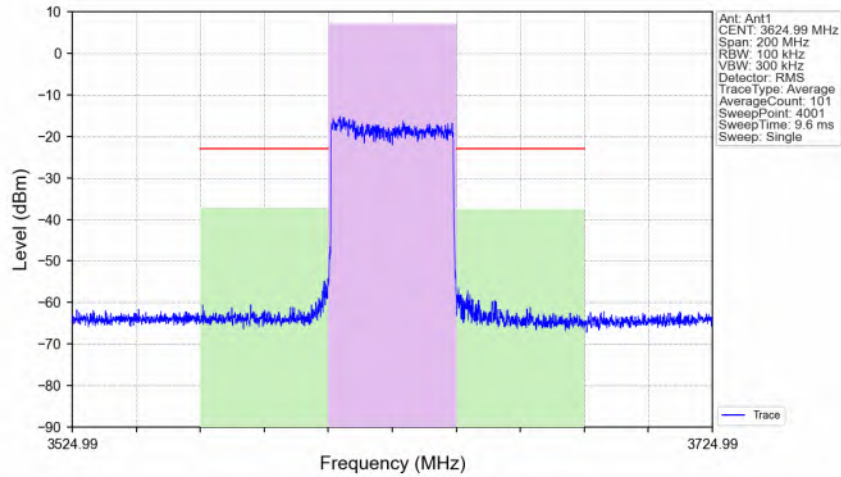
n48_30kHz_MIMO_NTNV_40MHz_CP-OFDM 16 QAM 3624.99MHz_Outer_Full_Ant1
