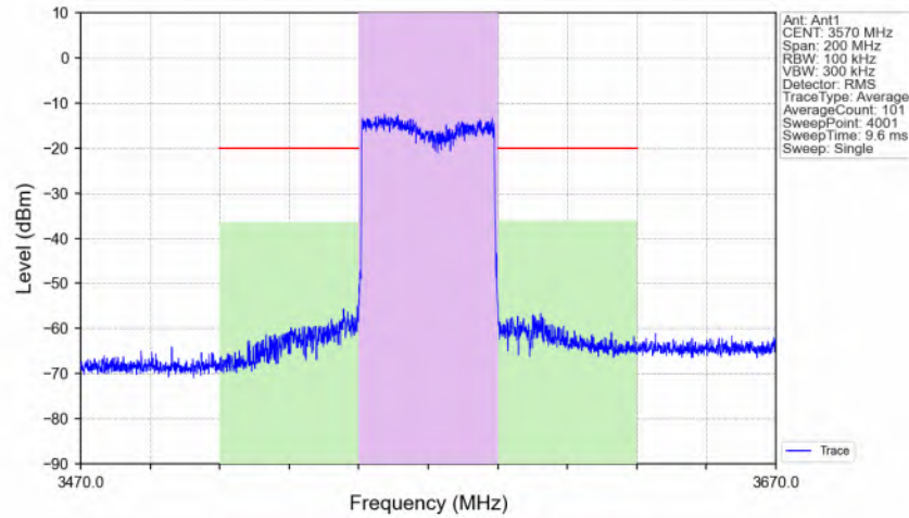
n48_30kHz_SISO_NTNV_40MHz_CP-OFDM 256 QAM 3570MHz_Outer_Full_Ant1
