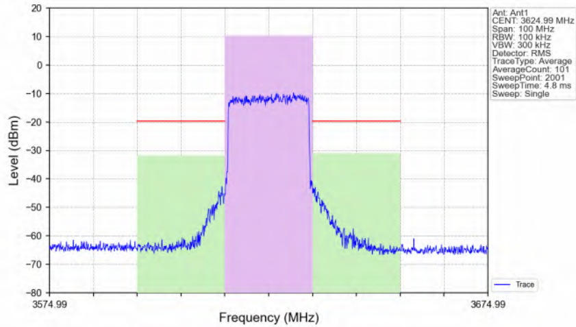
n48_30kHz_MIMO_NTNV_20MHz_CP-OFDM 16 QAM 3624.99MHz_Outer_Full_Ant1
