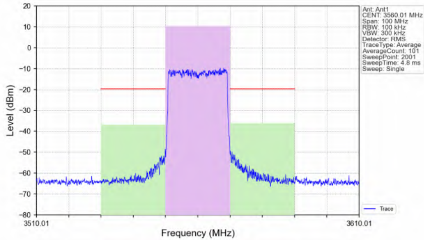
n48_30kHz_MIMO_NTNV_20MHz_CP-OFDM 64 QAM_3560.01MHz_Outer_Full_Ant1
