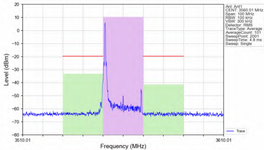
n48_30kHz_MIMO_NTNV_20MHz_CP-OFDM 64 QAM_3560.01MHz_Edge_1RB_Left_Ant1
