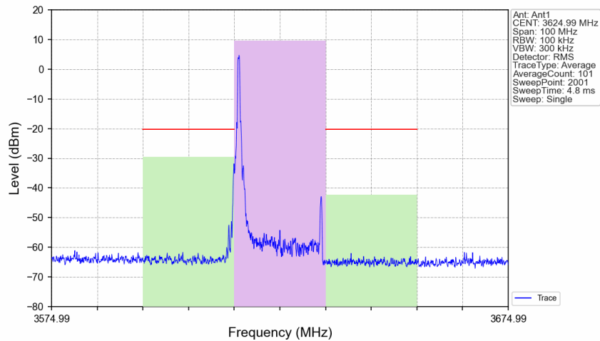
n48_30kHz_MIMO_NTNV_20MHz_CP-OFDM 16 QAM 3624.99MHz_Edge_1RB_Left_Ant1
