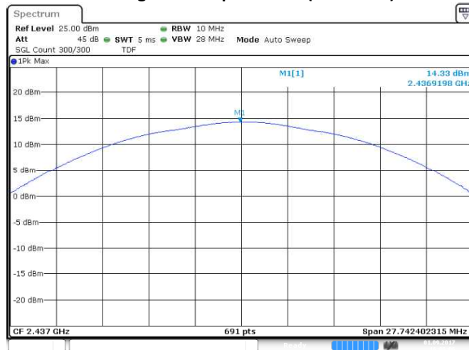
802.11g Peak Output Power (Channel 6)
