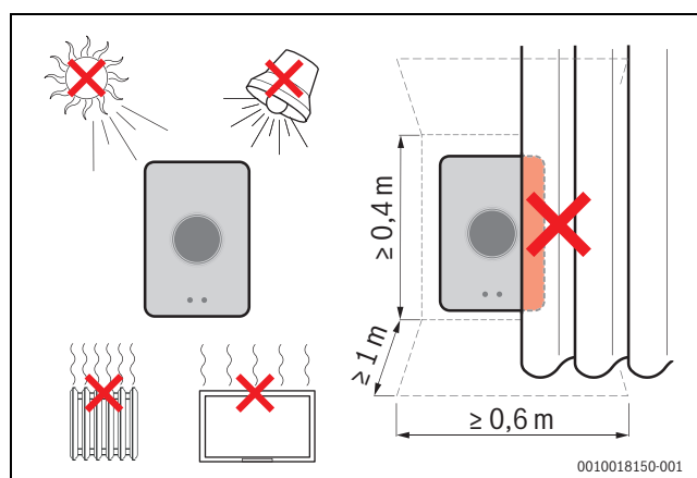
Fig. 4 Installation location for controller, condition
