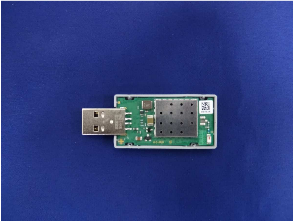
Photo 5: EUT Open View
