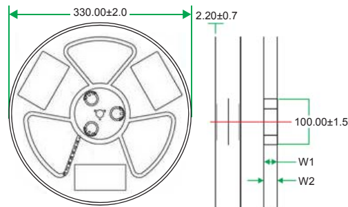
Figure 7-3. Reel Specification
