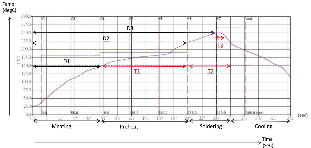
Figure 6-6. Reflow Profile for the Module
