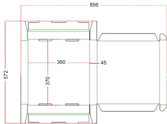
Figure 7-4. Reel Box
