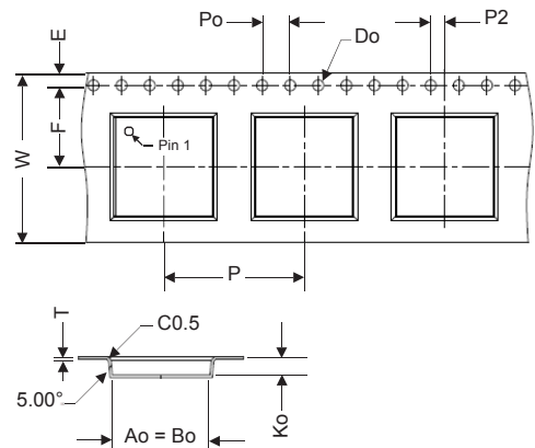
Figure 7-2. Tape Specification
