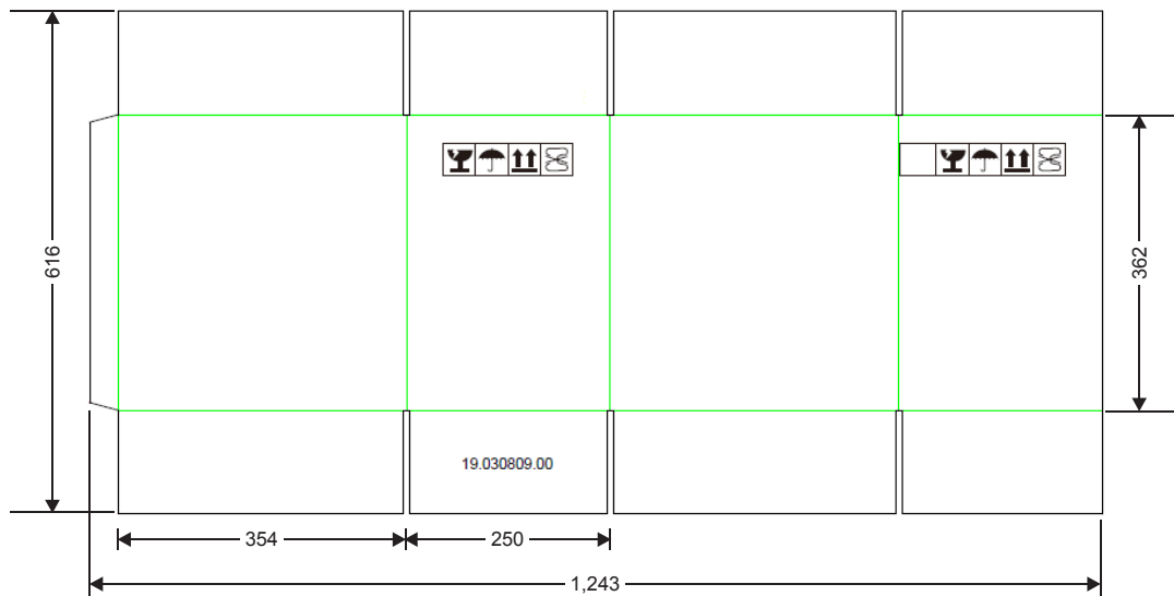
Figure 7-5. Shipping Box
