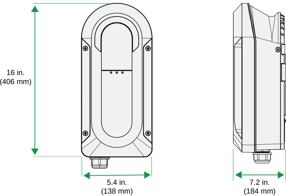
Figure 8 Dimensions
