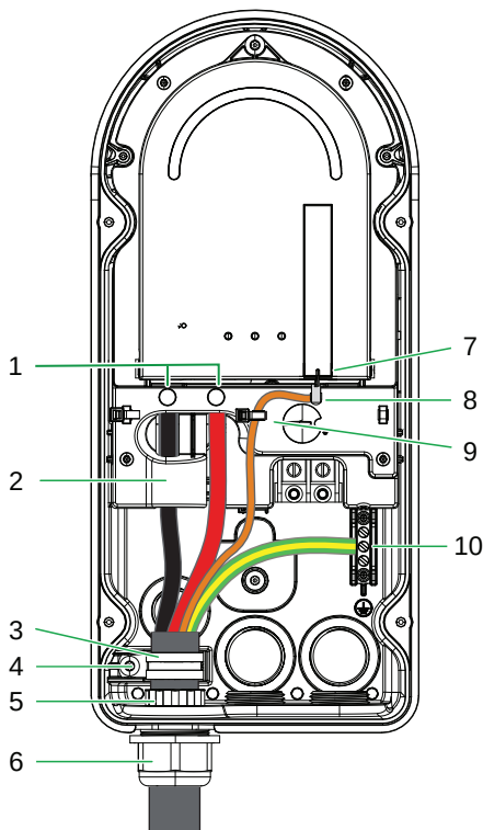
Figure 33 Pre-installed charging cable features (AC wiring excluded)
