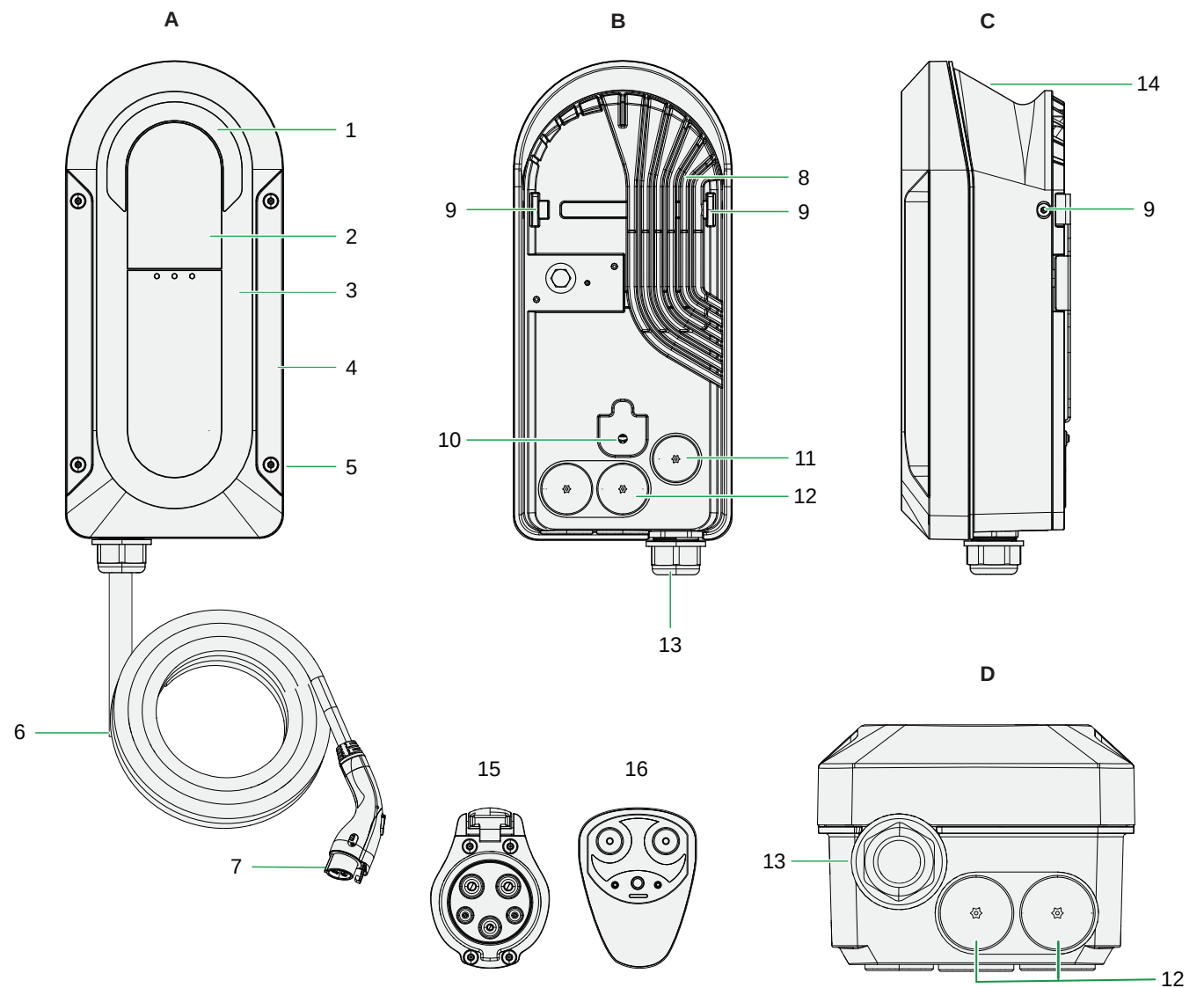
Figure 6 Physical features
