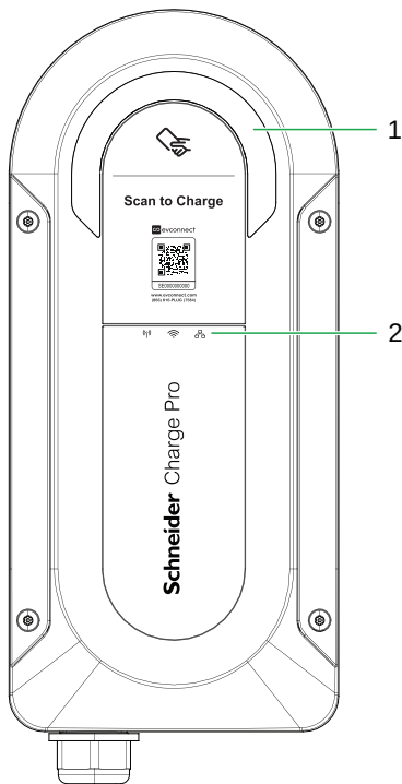
Figure 31 LED locations
