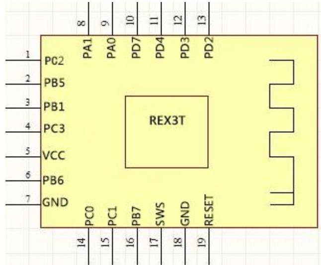
Figure 3-3. Pin Configuration
