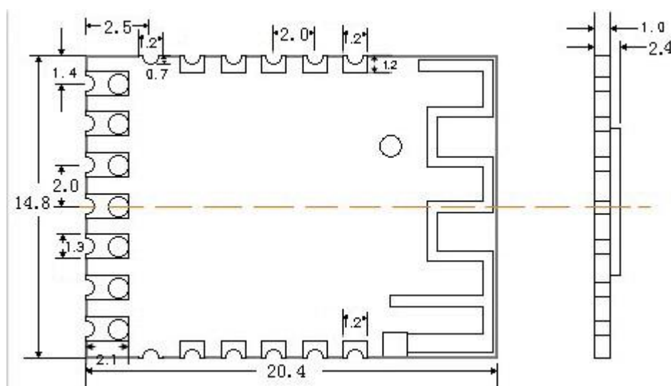
Figure3-1.Layout Dimension
