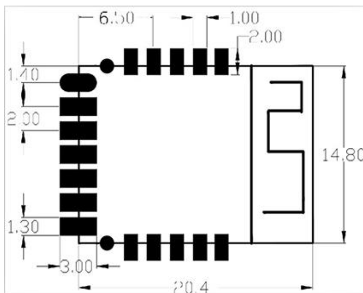
Figure3-2. Product Packages
