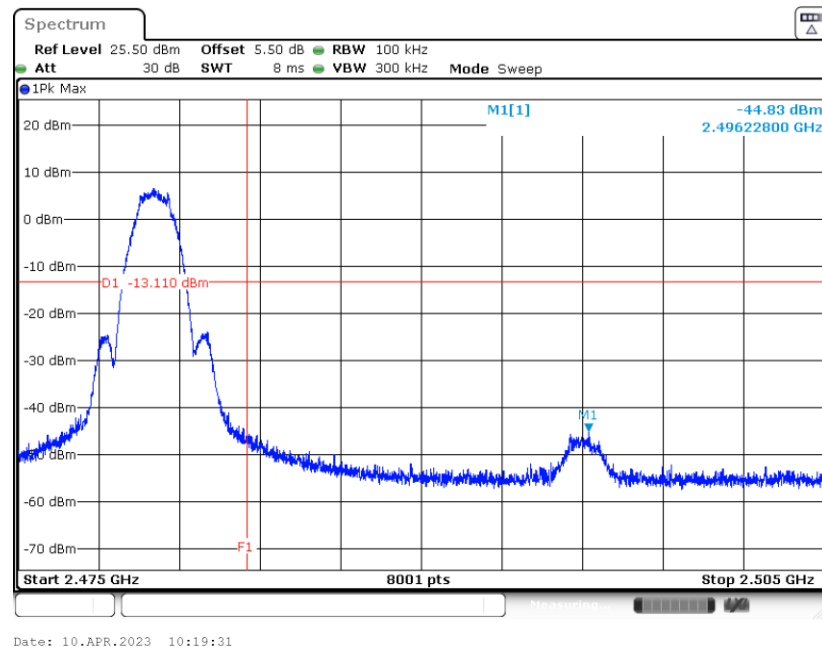
High Band Edge Plot on Channel 26
