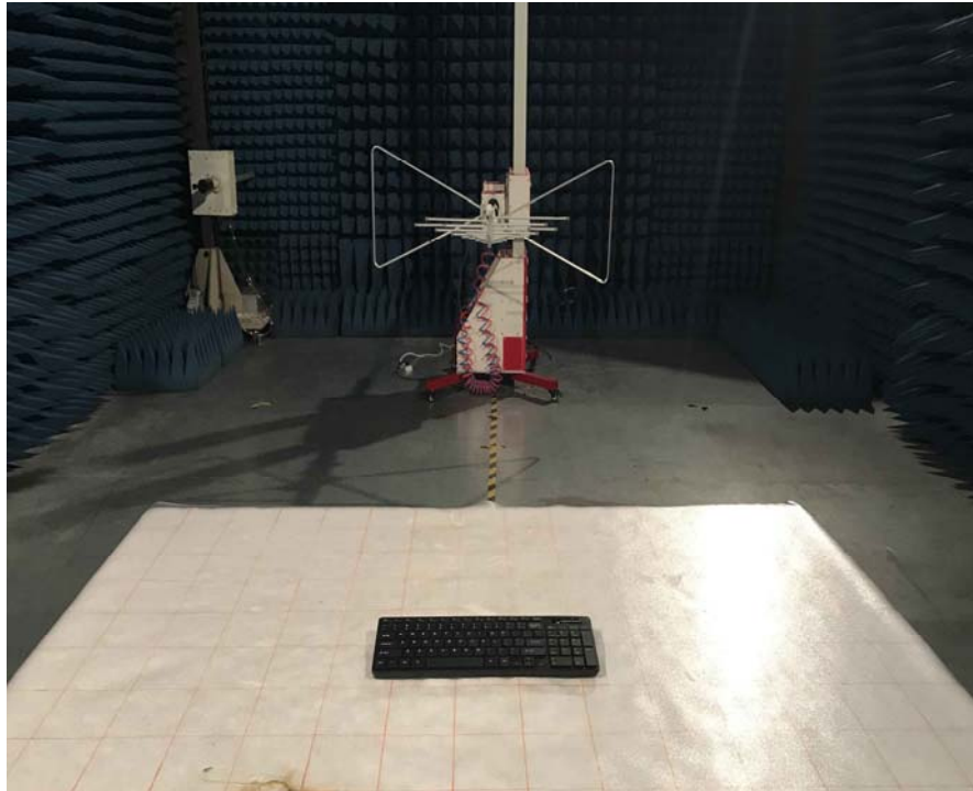
Product: 2.4G WIRELESS KEYBOARD Model: RK-8801 Radiated Emission
