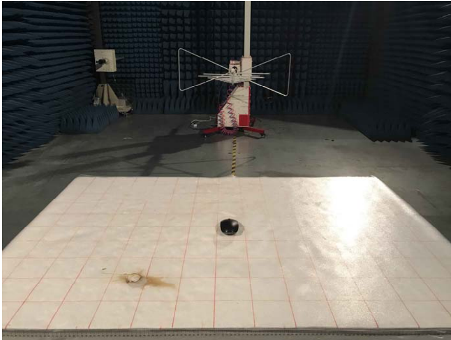
Product: 2.4G WIRELESS MOUSE Model: RM-8801 Radiated Emission
