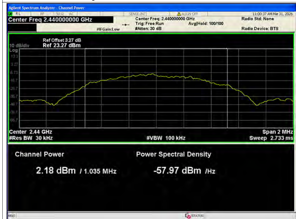
Average Power NVNT BLE 1M 2440MHz Ant2
