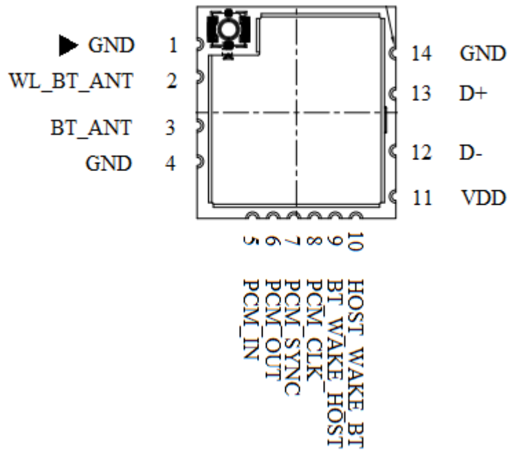
Figure 2.2 Pin Outline
