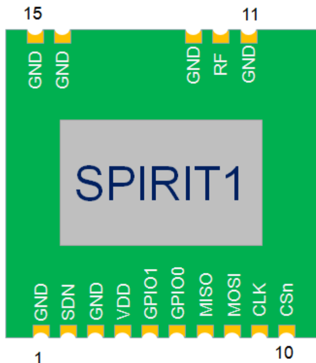
Figure 2 Module Pin Definition
