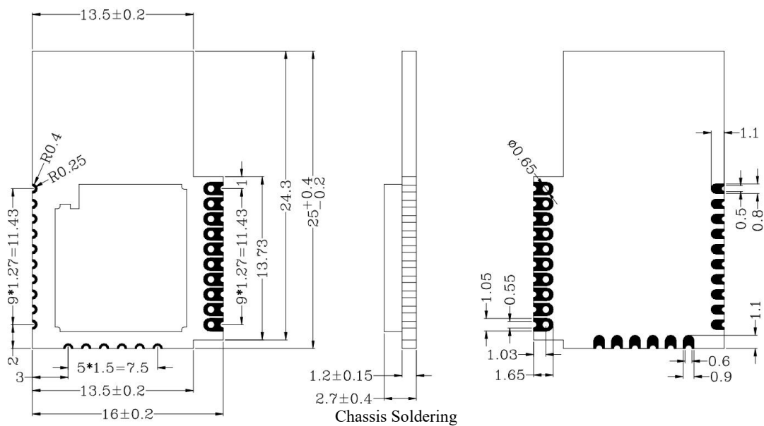
Fig. 2-2 Dimensional Drawing of LSD4BT-K53ASTD001
