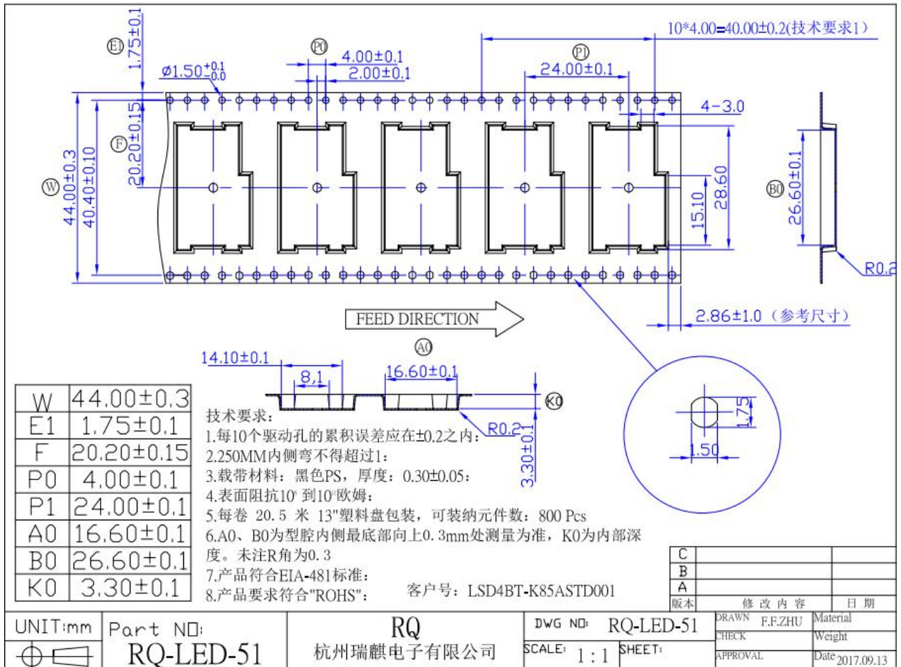
Fig. 6-1 Package Size
