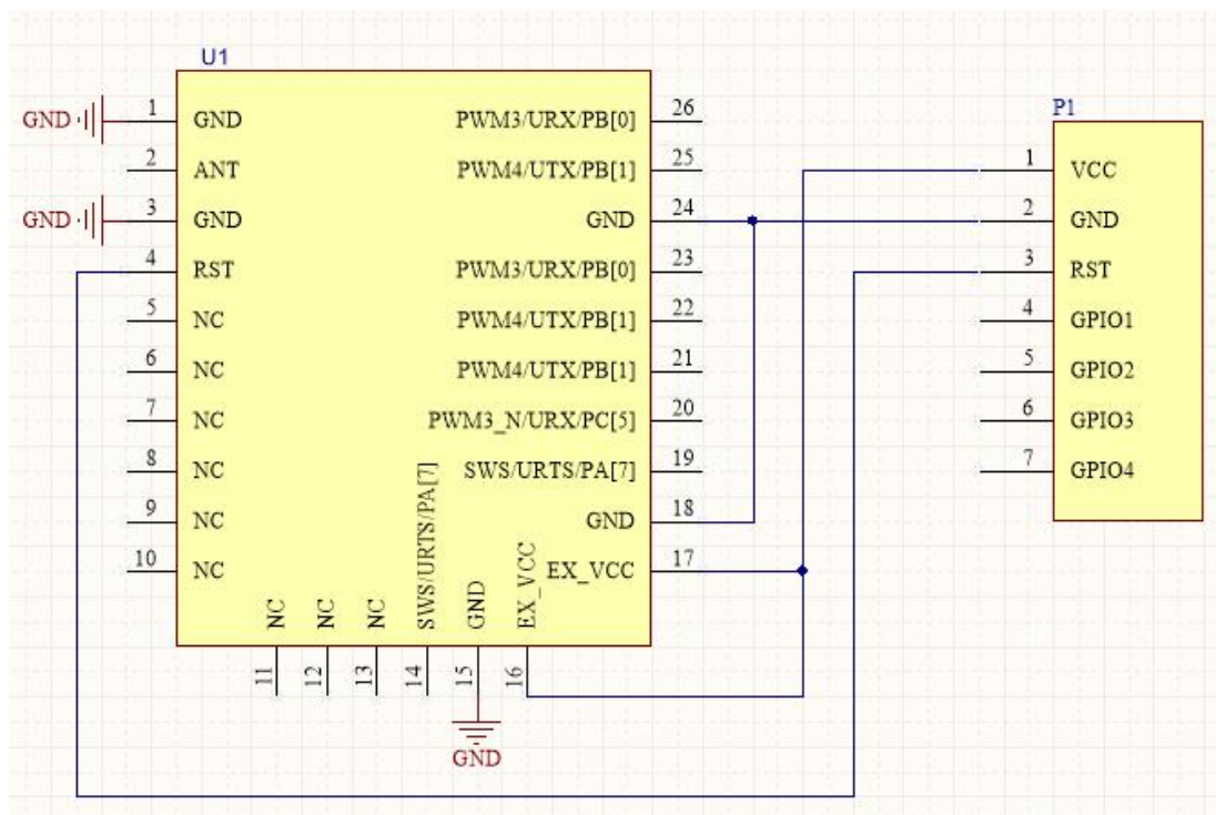
Fig. 3-1 Typical Application Circuits
