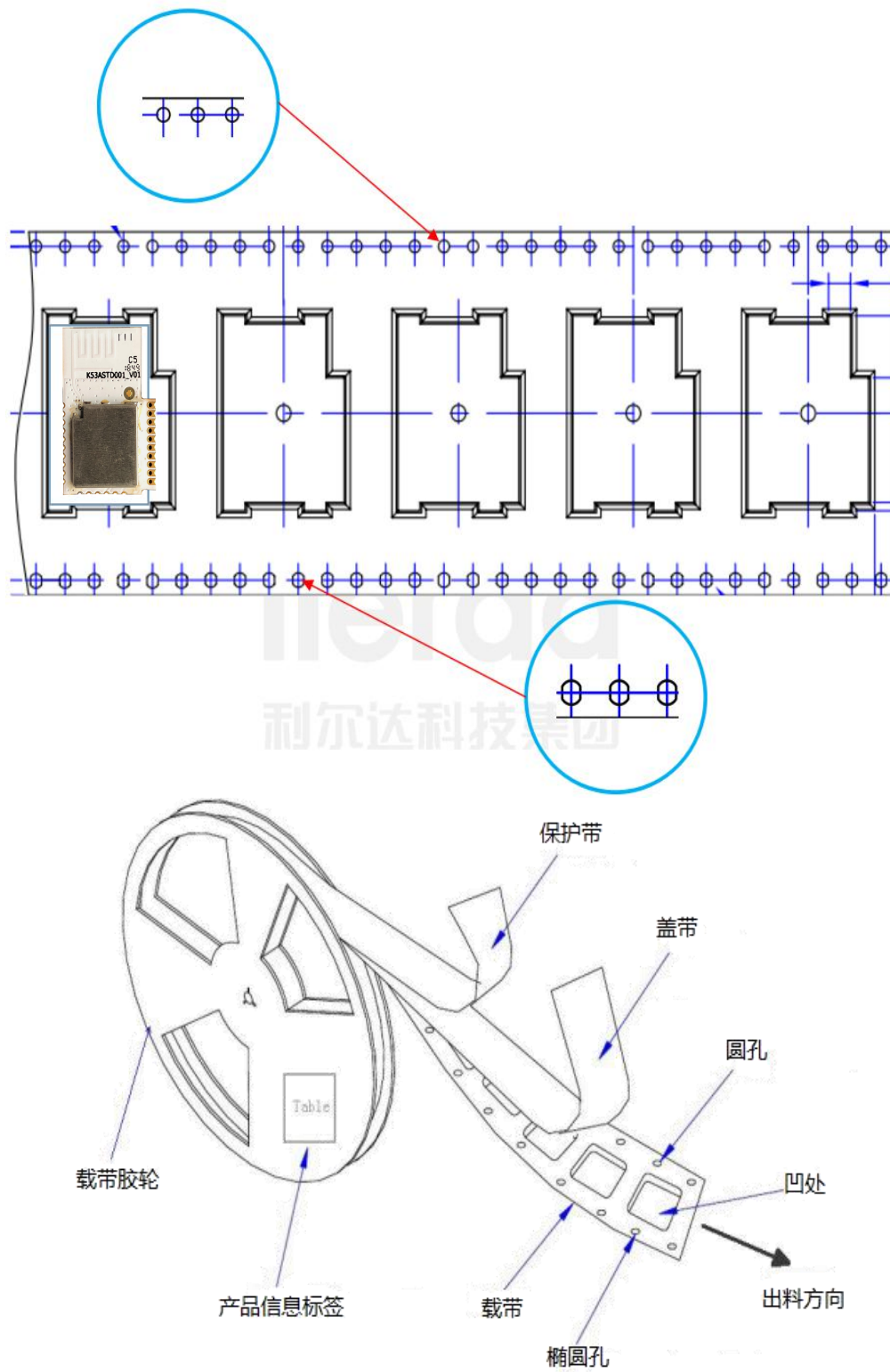
Fig. 6-2 Packaging Direction
