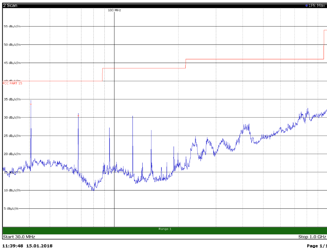
Figure 8.3-2: Field strength of spurious emissions above 30 MHz – Antenna in horizontal polarization
