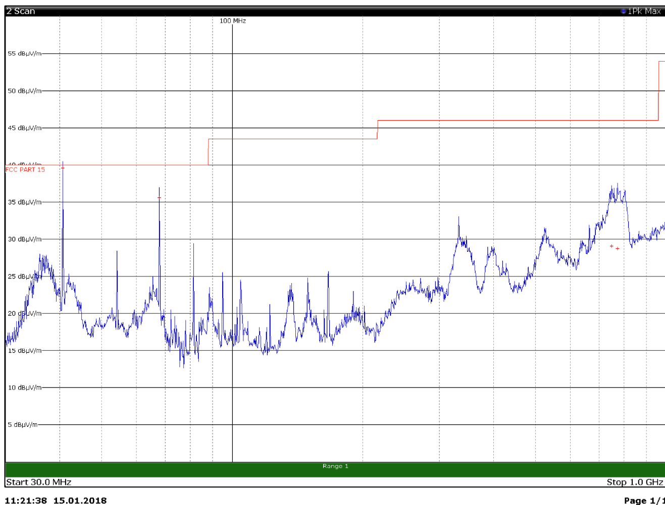
Figure 8.3-3: Field strength of spurious emissions above 30 MHz – Antenna in vertical polarization
