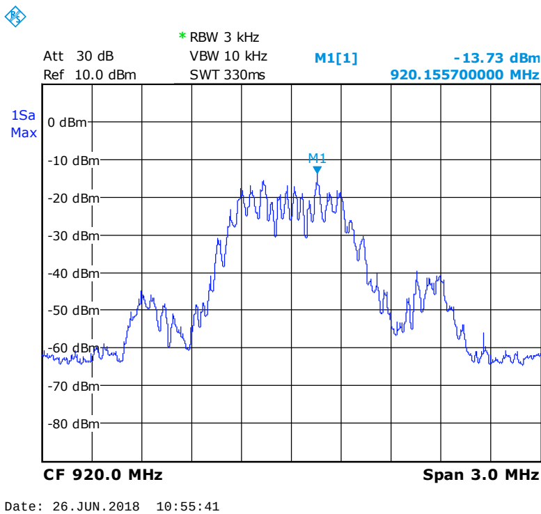
Figure 4.6.1 Measurement of power spectral density.
