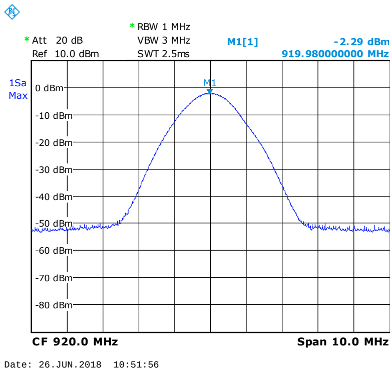
Figure 4.3.1 Maximum conducted output power. Nominal temperature and voltage.
