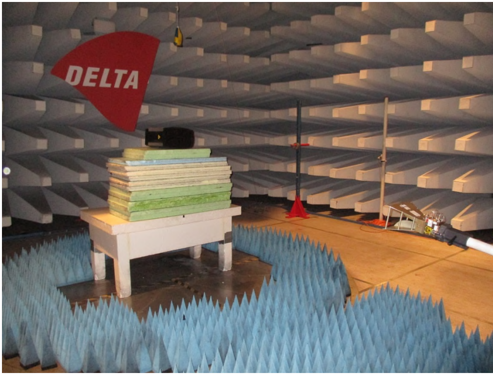
Photo 4.2.3 Test setup regarding measurement of radio frequency electromagnetic field (above 1 GHz). Horizontal orientation of test object
