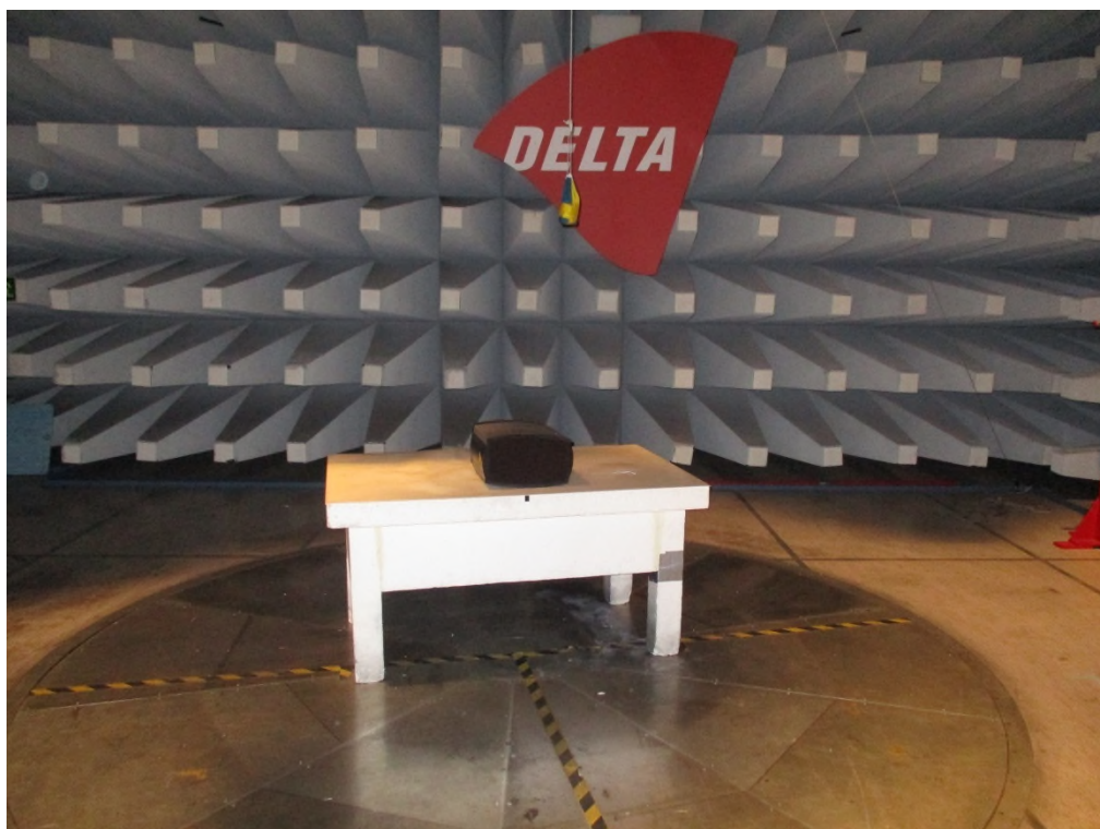
Photo 2.3 Test set up regarding measurement of radio frequency electromagnetic field below 1 GHz. Horizontal orientation
