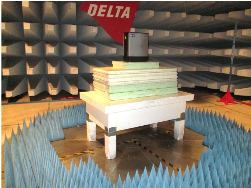
Photo 2.5 Test set up regarding measurement of radio frequency electromagnetic field above 1 GHz.
