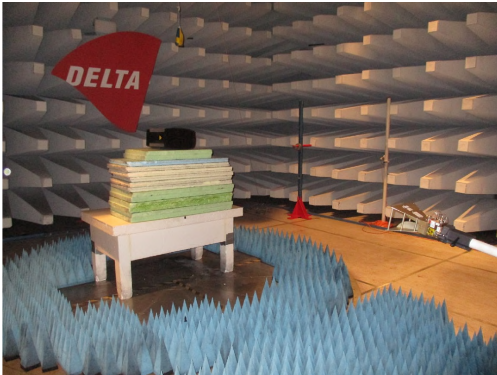
Photo 2.7 Test set up regarding measurement of radio frequency electromagnetic field above 1 GHz. Horizontal orientation
