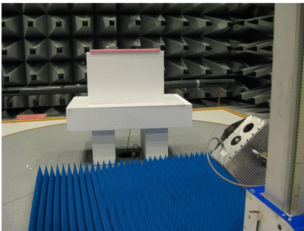
Photo 4.5.1 Test setup regarding measurement of radio frequency electromagnetic field (above 1 GHz).
