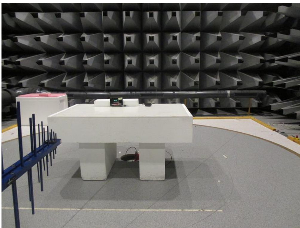
Photo 4.4.1 Test setup regarding measurement of radio frequency electromagnetic field.
