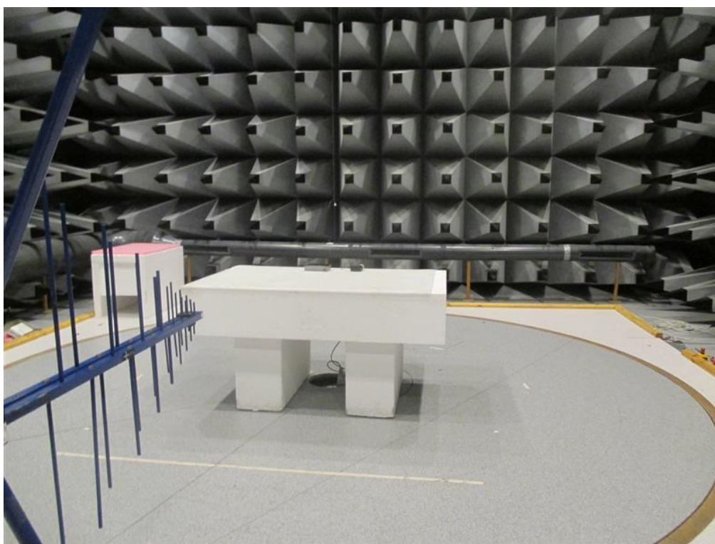
Photo 4.3.1 Test setup regarding measurement of radio frequency electromagnetic field.
