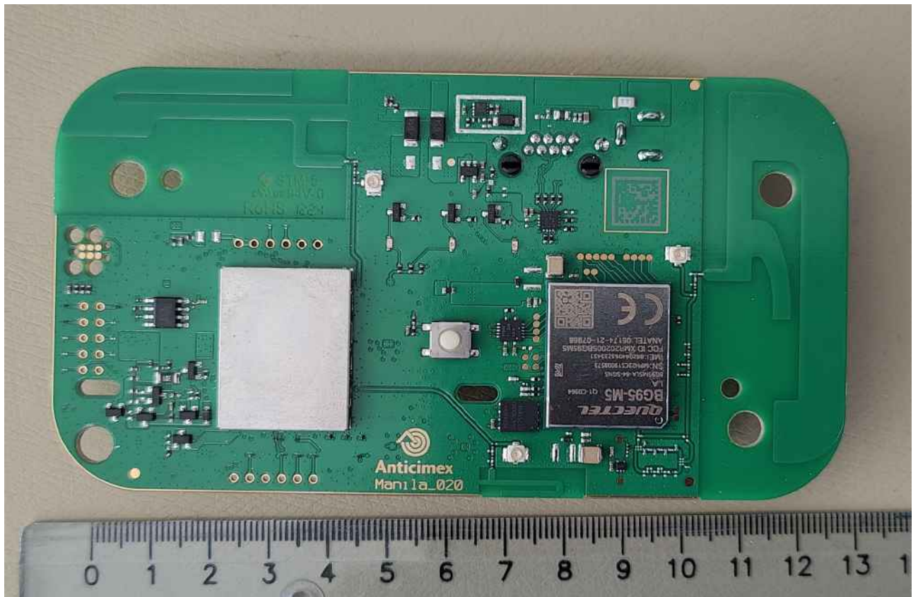
EUT PCB from front side
