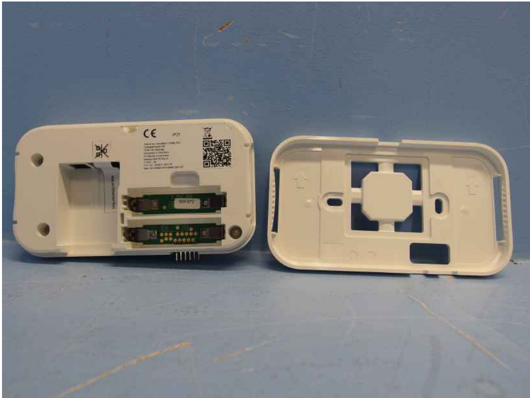
EUT rear side and the inside of wall bracket
