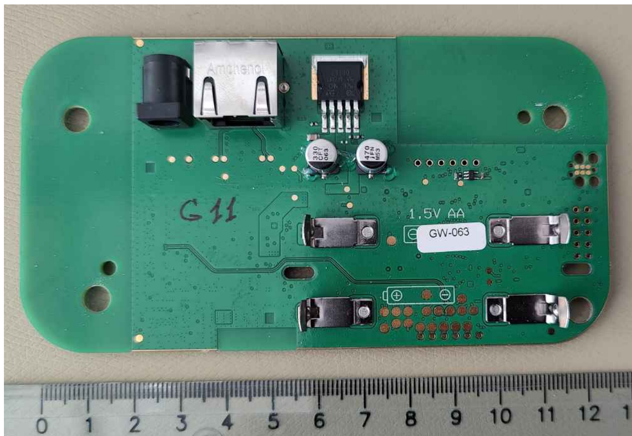
EUT PCB from bottom side
