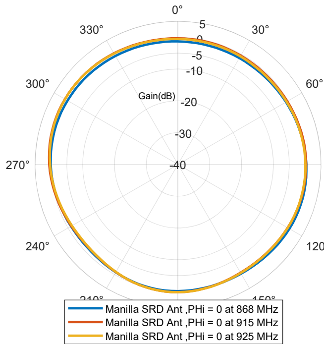
Antenna Gain in Elevation plane,(X-Z plane)
