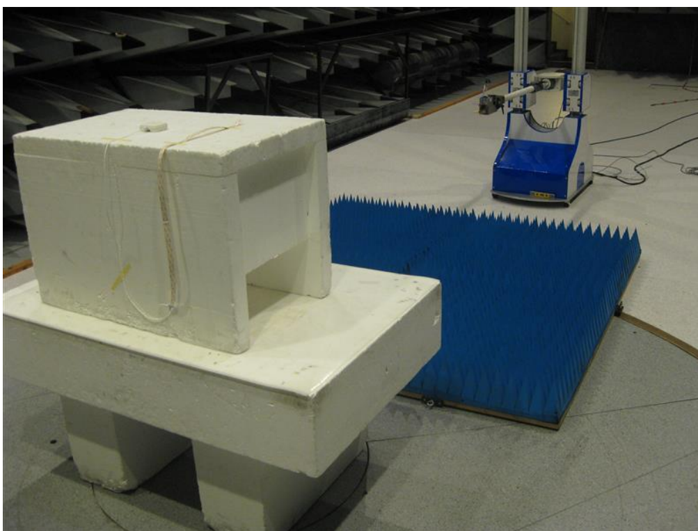
Photo 4.10.2 Test set-up regarding measurement of radiated emission (above 1 GHz).
